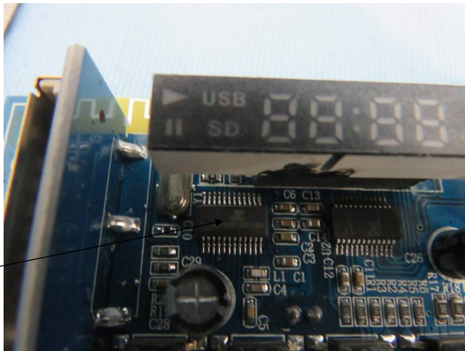
RF Chip
