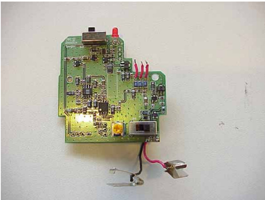
Photo No. 5 TOP VIEW OF PCB1
