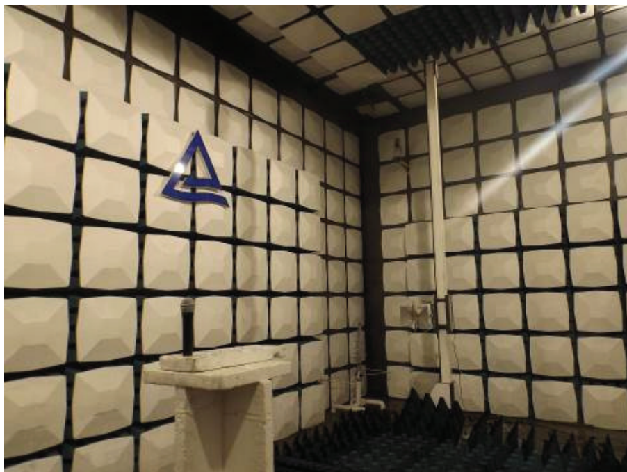
Picture 2: Spurious Radiation Measurement, Above 1GHz (CH99)
