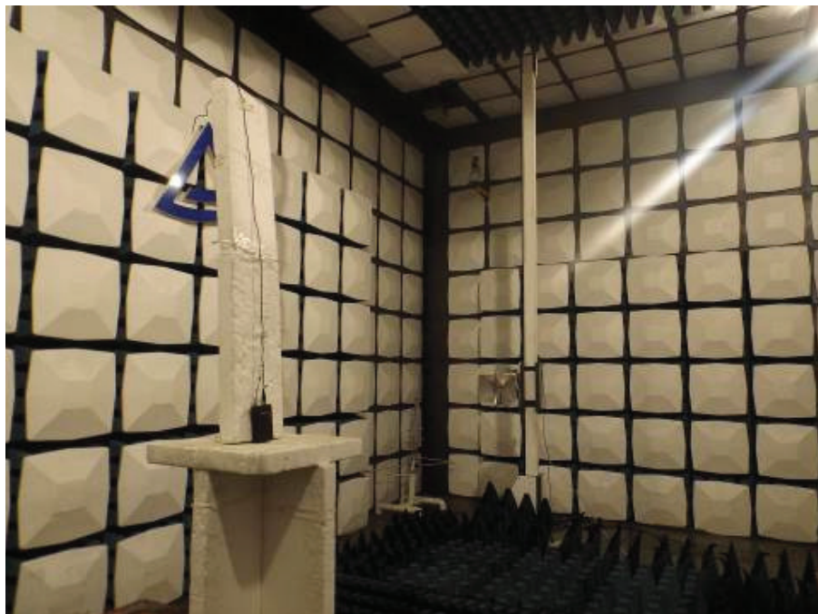
Picture 2: Spurious Radiation Measurement, Above 1GHz (CB99)
