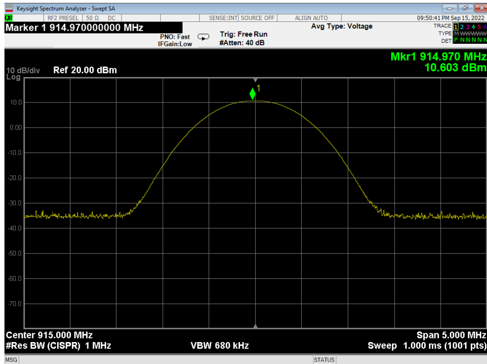
Figure 6 – Output Power, Mid Channel
