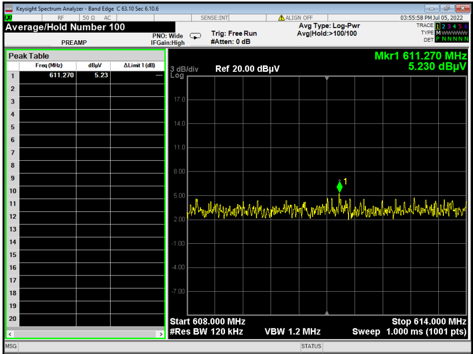
Figure 12 - Band-edge Measurement, Low Channel, Restricted Frequency, Continuous
