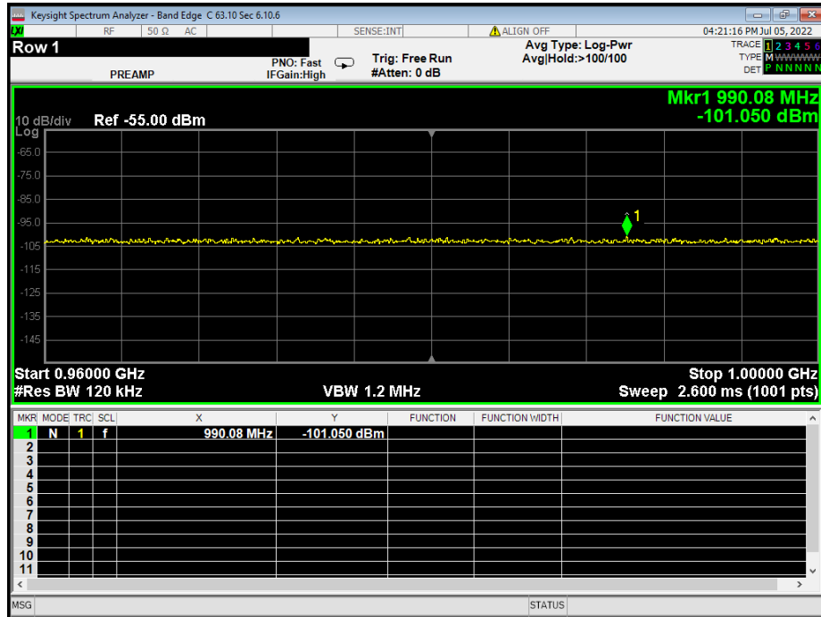
Figure 15 - Band-edge Measurement, High Channel, Restricted Frequency, Continuous
