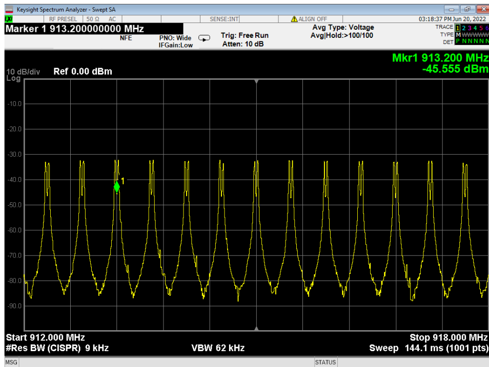
Figure 23 – Hop Count, 912-918MHz
