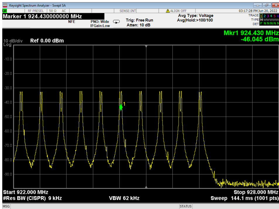
Figure 25 – Hop Count, 922-928MHz
