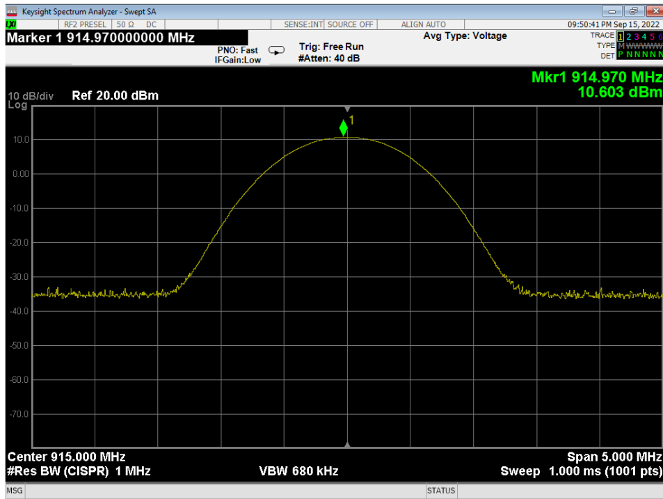
Figure 7 – Output Power, High Channel *See Section 4.0 for included corrections
