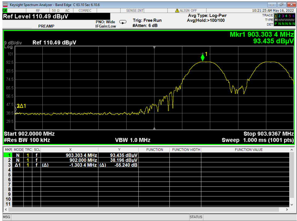
Figure 14 - Band-edge Measurement, Low Channel, Unrestricted Frequency, Hopping The plot shows a corrected measurement, used for relative measurements only.
