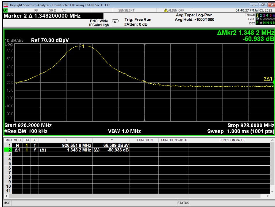
Figure 16 - Band-edge Measurement, High Channel, Unrestricted Frequency, Continuous The plot shows an uncorrected measurement, used for relative measurements only.
