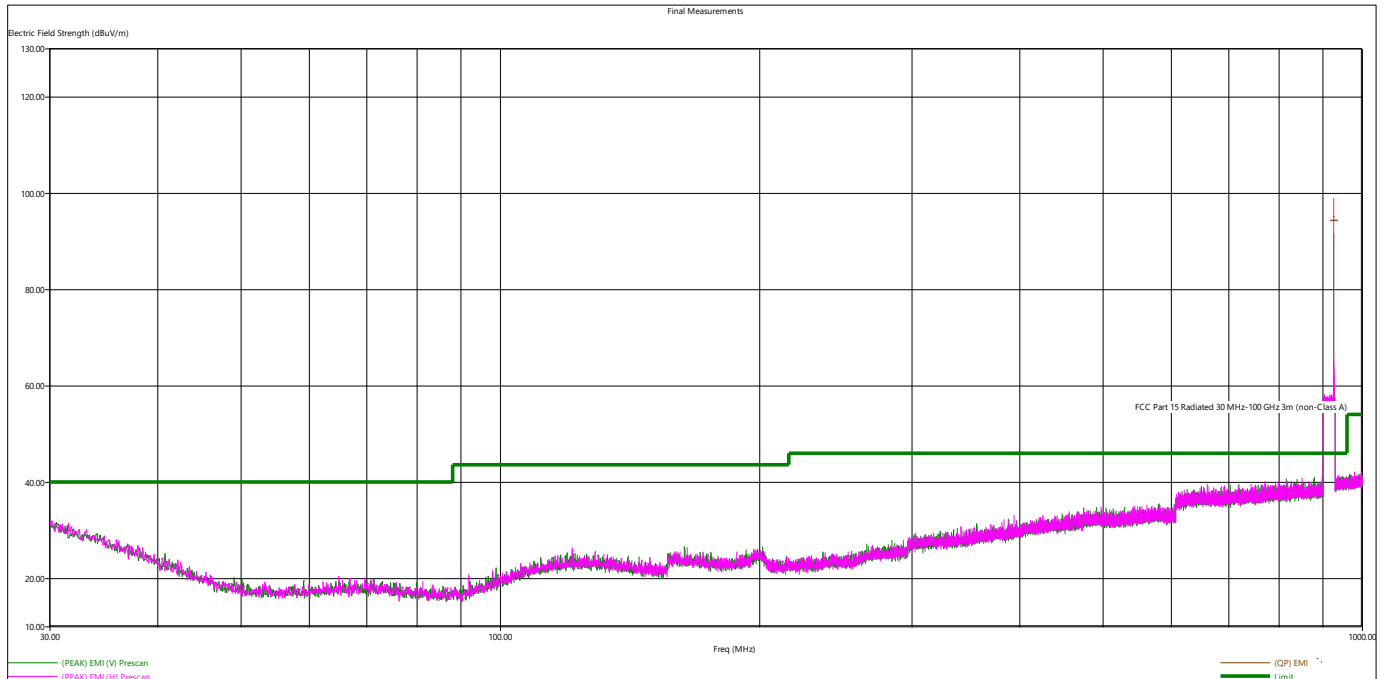
Figure 4 - Radiated Emissions Plot, 30 MHz-1 GHz High Channel
