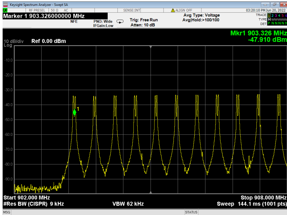
Figure 21 – Hop Count, 902-908MHz
