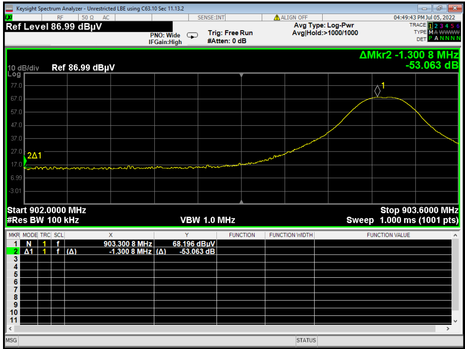
Figure 13 - Band-edge Measurement, Low Channel, Unrestricted Frequency, Continuous The plot shows an uncorrected measurement, used for relative measurements only.
