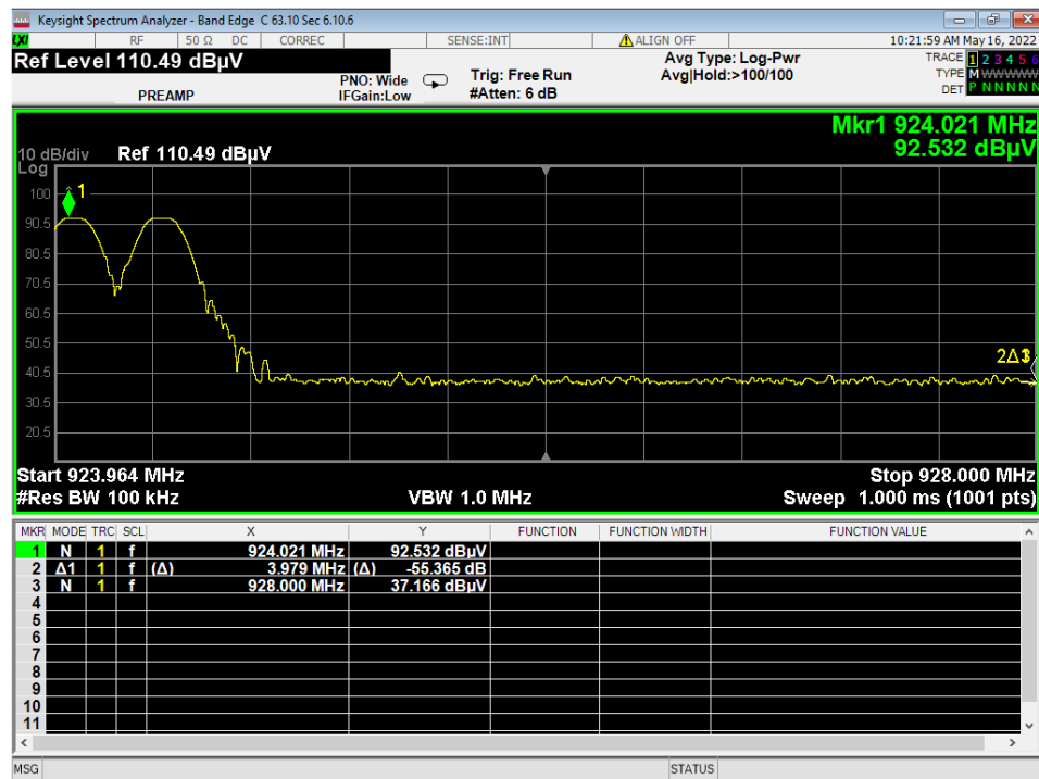
Figure 17 - Band-edge Measurement, High Channel, Unrestricted Frequency, Hopping The plot shows a corrected measurement, used for relative measurements only.
