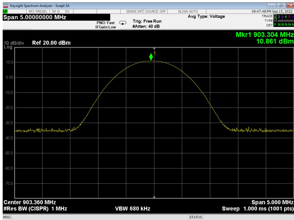
Figure 5 – Output Power, Low Channel.
