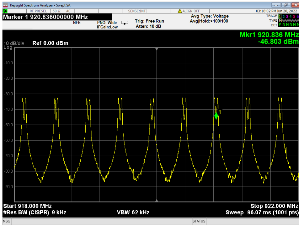
Figure 24 – Hop Count, 918-922MHz
