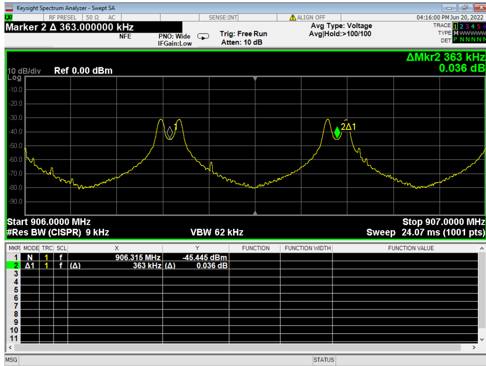
Figure 20 – Minimum Frequency Separation, 363.0 kHz
