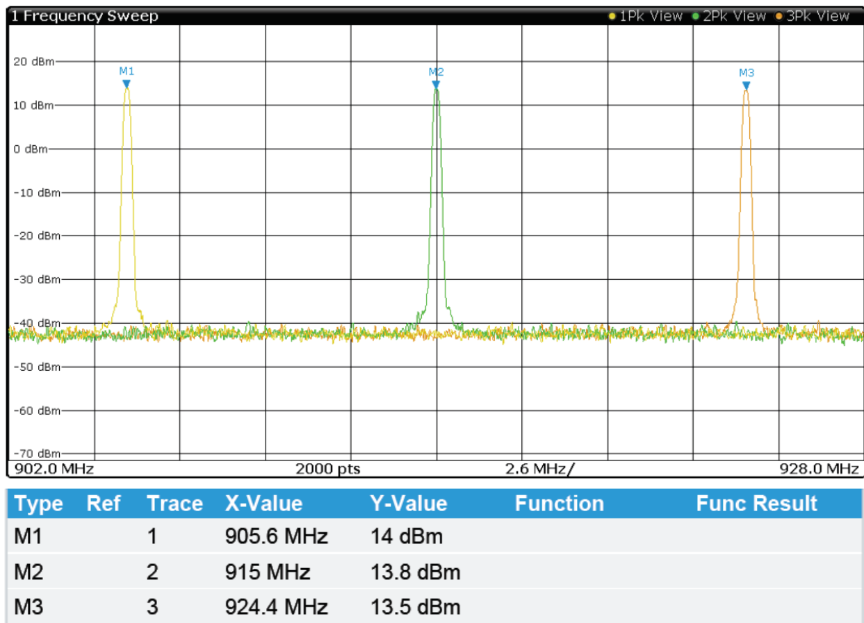
Figure 3 Plot of Transmitter Operation across 902-928 MHz
