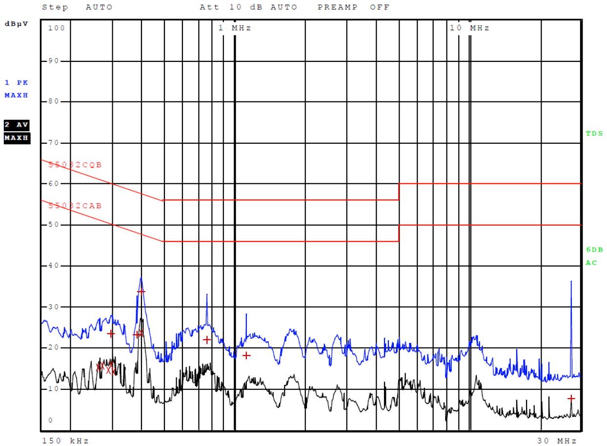
Figure 1 AC Line Conducted emissions of EUT line 1
