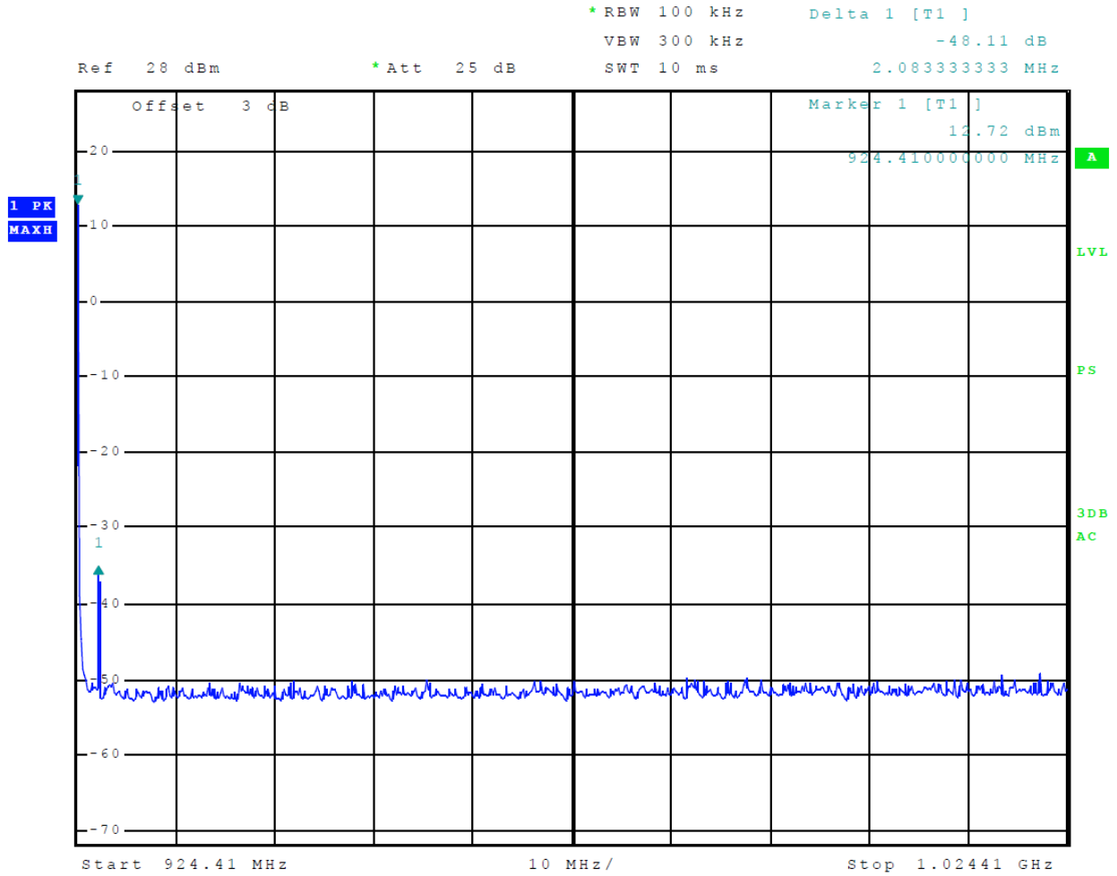
Figure 12 Plot of Transmitter Emissions High Band Edge Channels Hopping
