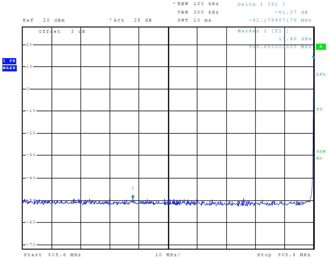
Figure 11 Plot of Transmitter Emissions Low Band Edge Channels Hopping
