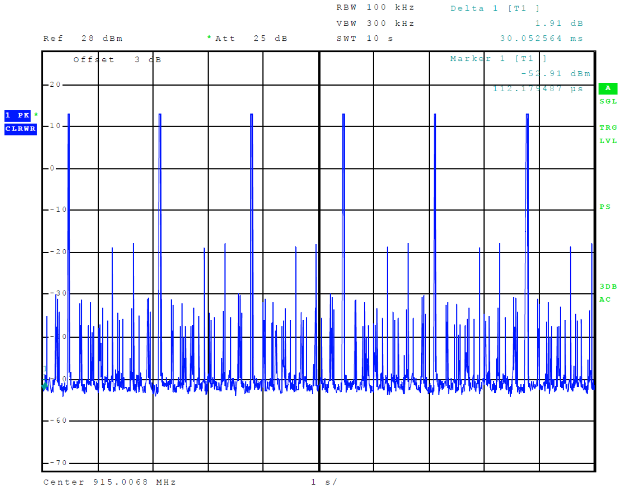
Figure 10 Plot of 6 Times on Channel over 10 second period
