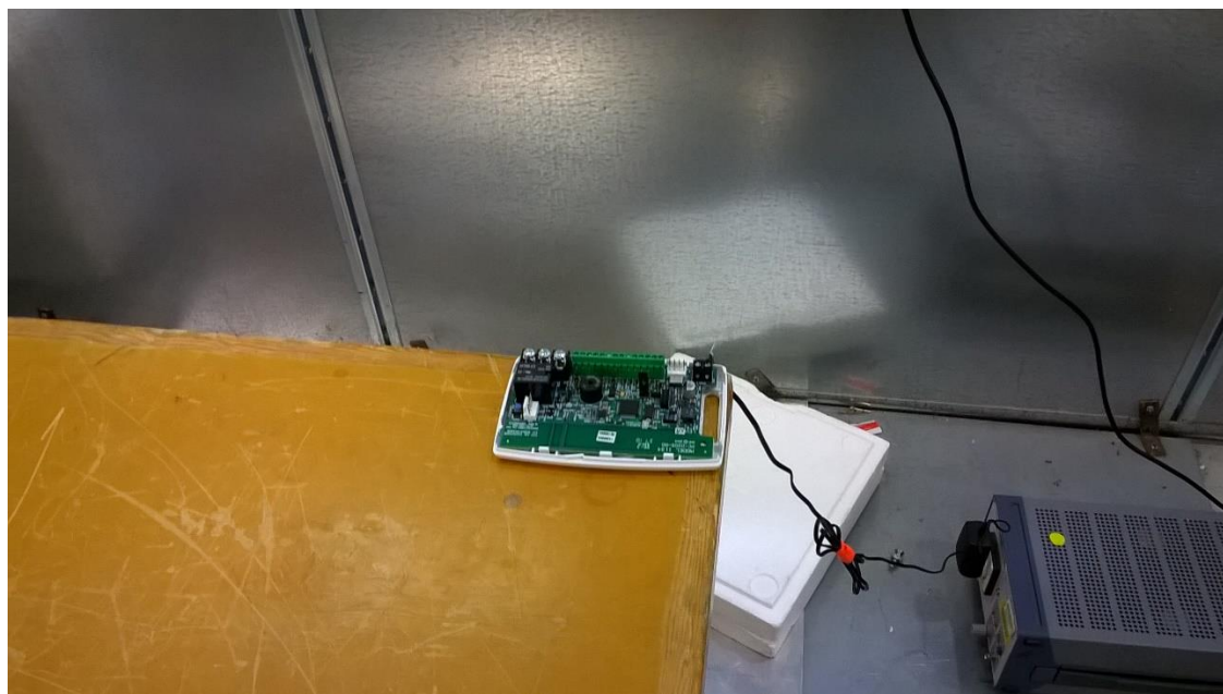
Figure 5 - Conducted emissions test setup, 150kHz - 30MHz
