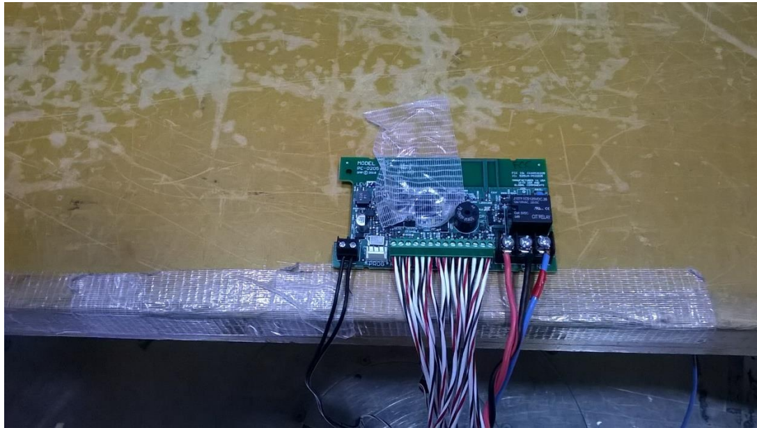
Figure 3 - Radiated emissions test setup - with IO ports populated
