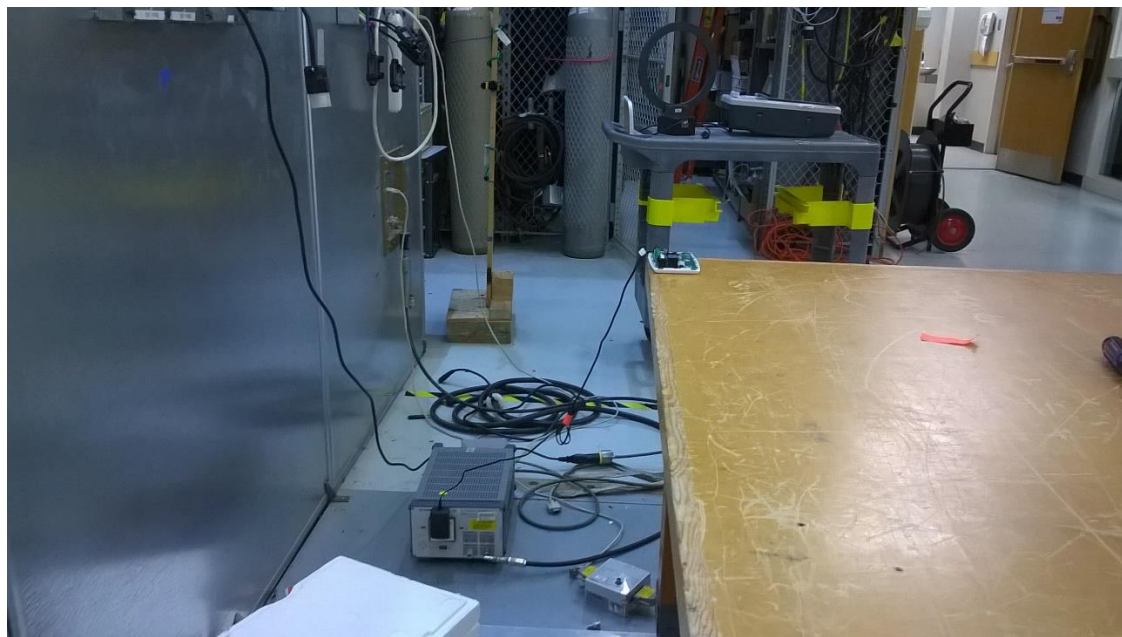
Figure 6 - Conducted emissions test setup, 150kHz - 30MHz
