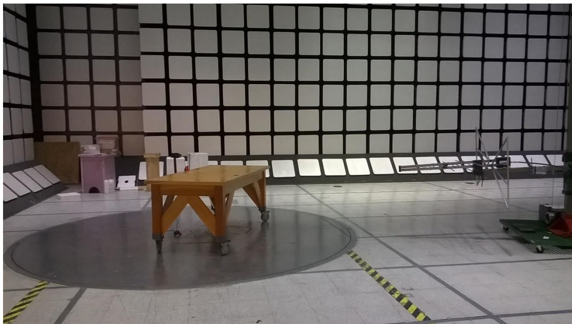
Figure 2 - Radiated emissions test setup, 30MHz - 1GHz
