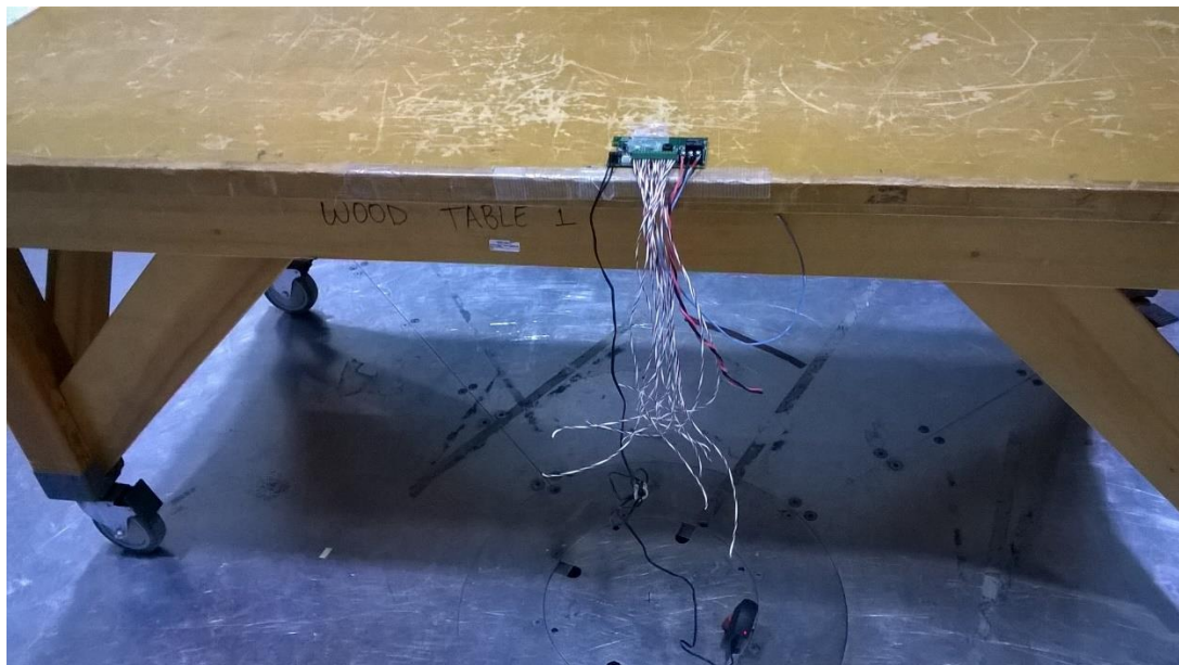
Figure 4 - Radiated emissions test setup - with IO ports populated
