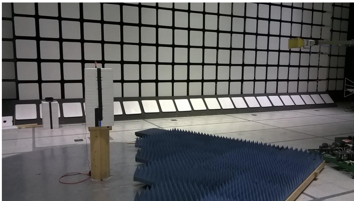
Figure 1 - Radiated emissions test setup, 1 - 18GHz
