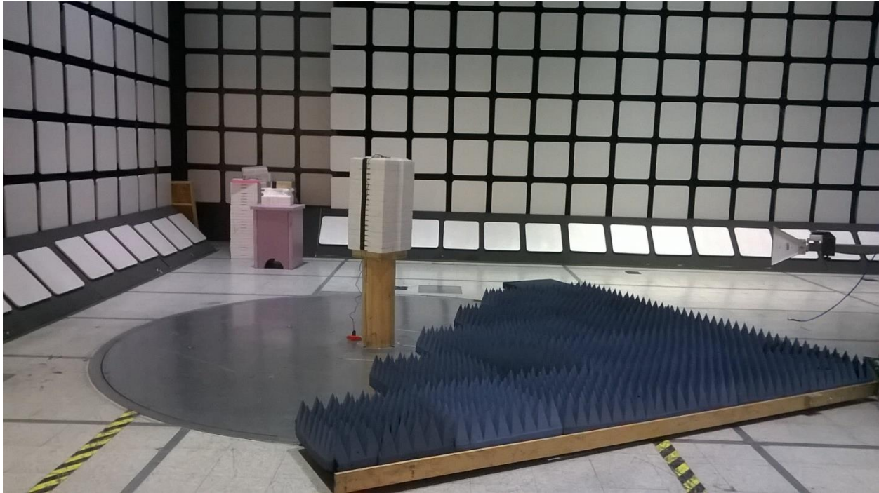
Figure 3 - Test Setup, 1 – 10GHz, X axis
