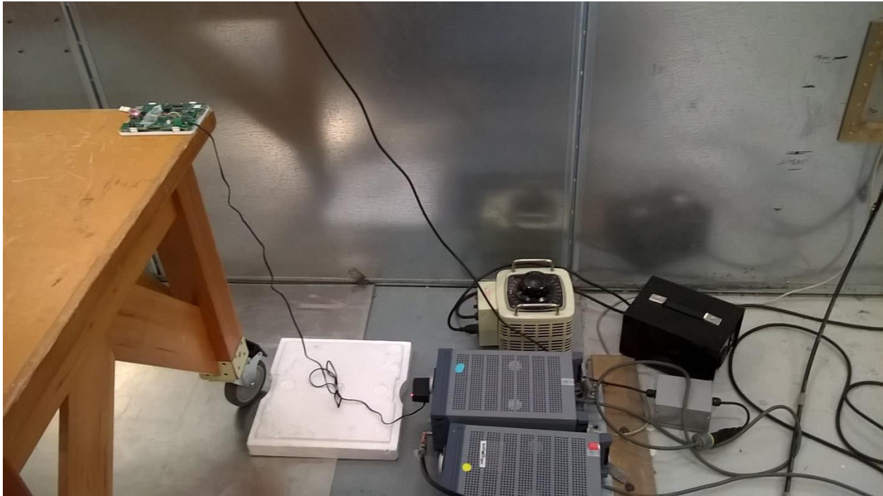
Figure 7 - Conducted Emissions Test Setup
