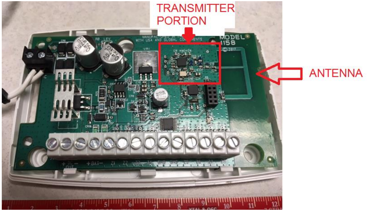
Figure 2 - Location of Antenna
