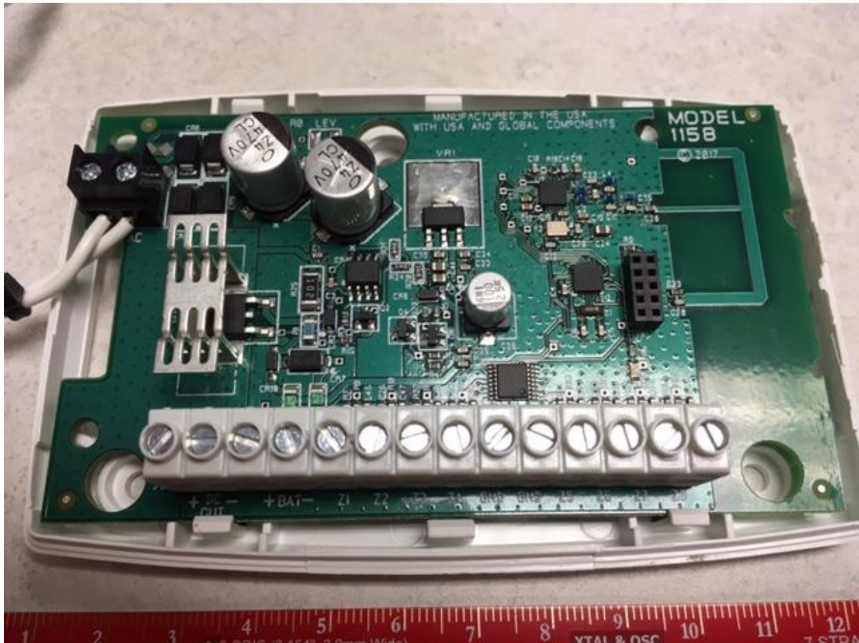
Figure 1 – Top of PCB inside case
