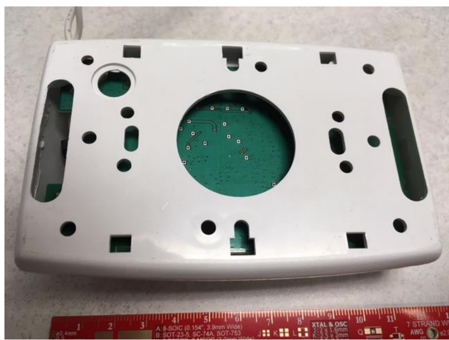
Figure 6 - Back of unit
