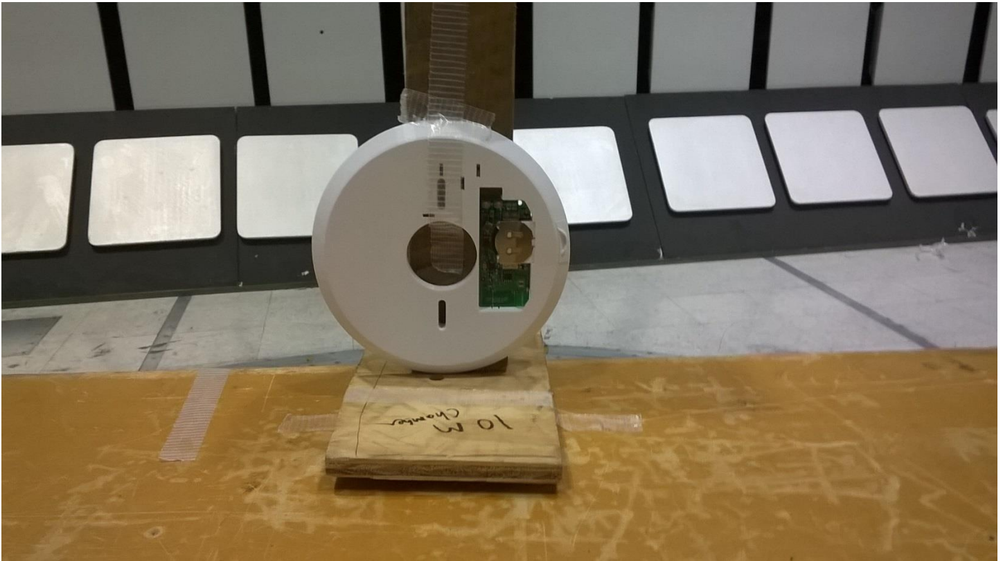
Figure 3 - Radiated emissions test setup, 30MHz - 1GHz, Z-axis
