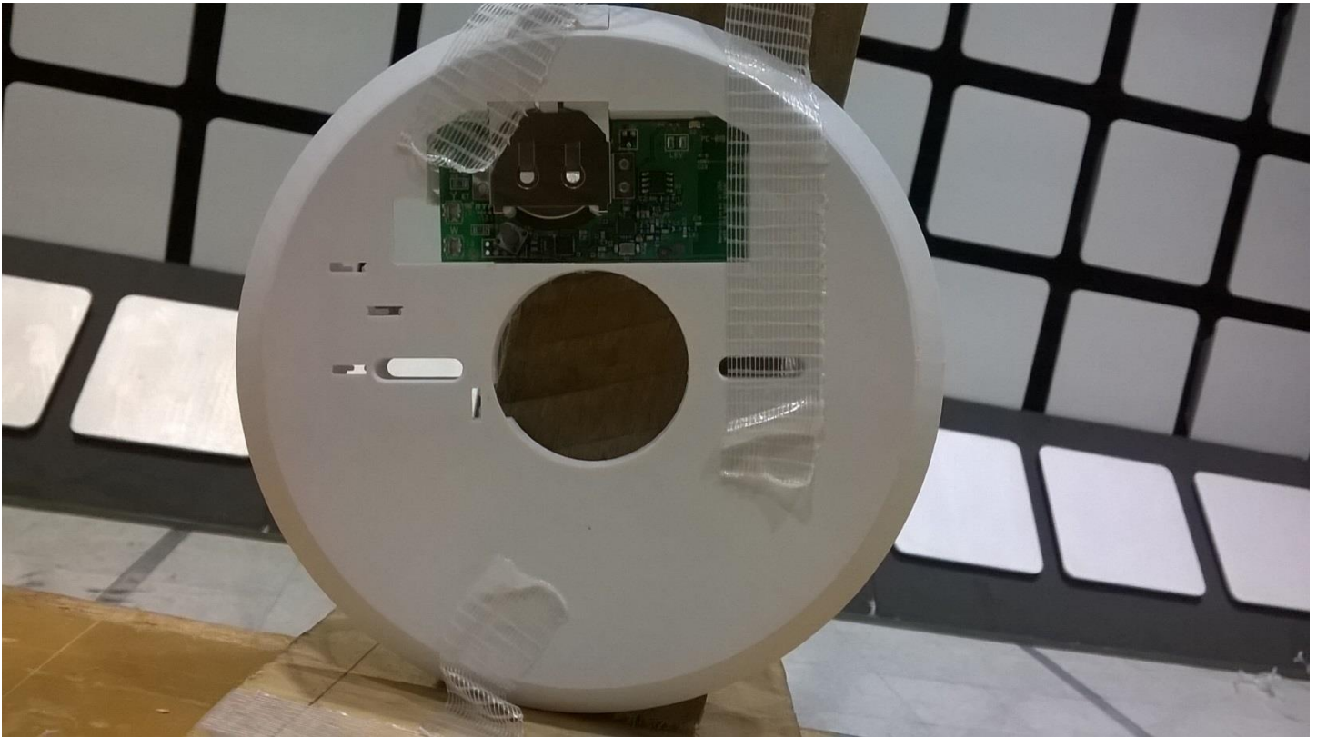
Figure 2 - Radiated emissions test setup, 30MHz - 1GHz, Y-axis
