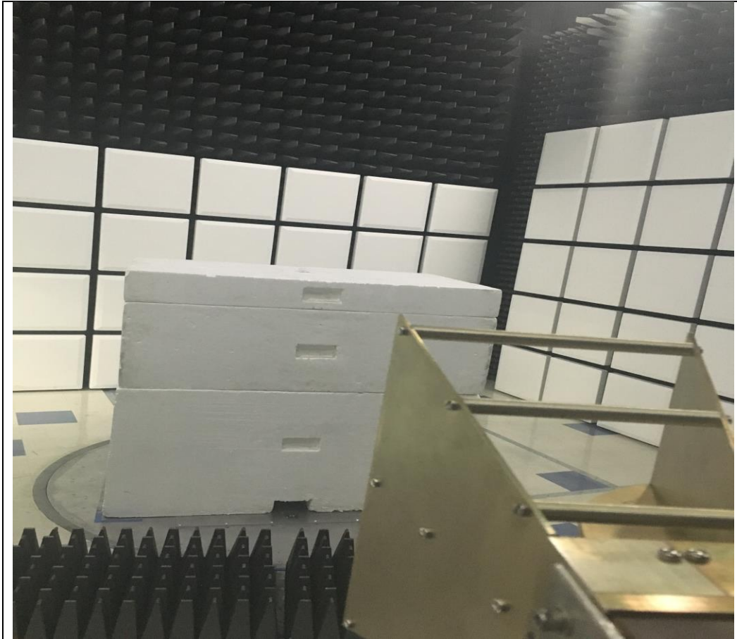
RF Radiated #1
