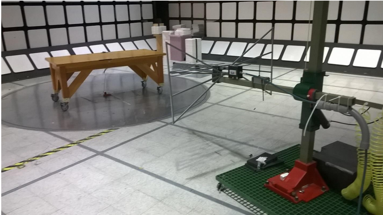
Figure 1 - Test Setup, 30MHz - 1GHz, X axis (testing was performed in all 3 axis for 30MHz – 1GHz measurements)
