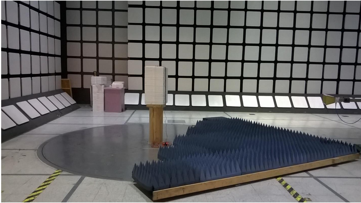
Figure 2 - Test Setup, 30MHz - 1GHz, X axis (testing was performed in all 3 axis for 30MHz – 1GHz measurements)
