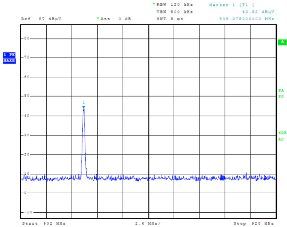
Figure Seven Plot of Operation in 902-928 MHz Frequency Band
