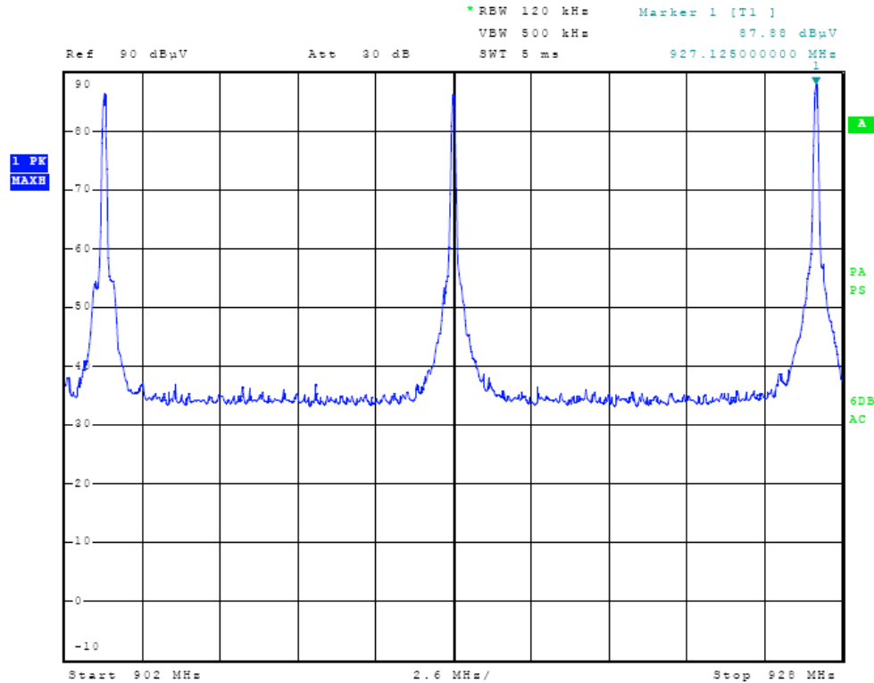
Figure Six Output power across band
