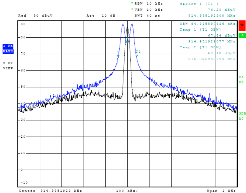
Figure Eight Occupied Bandwidth (Mid Channel)
