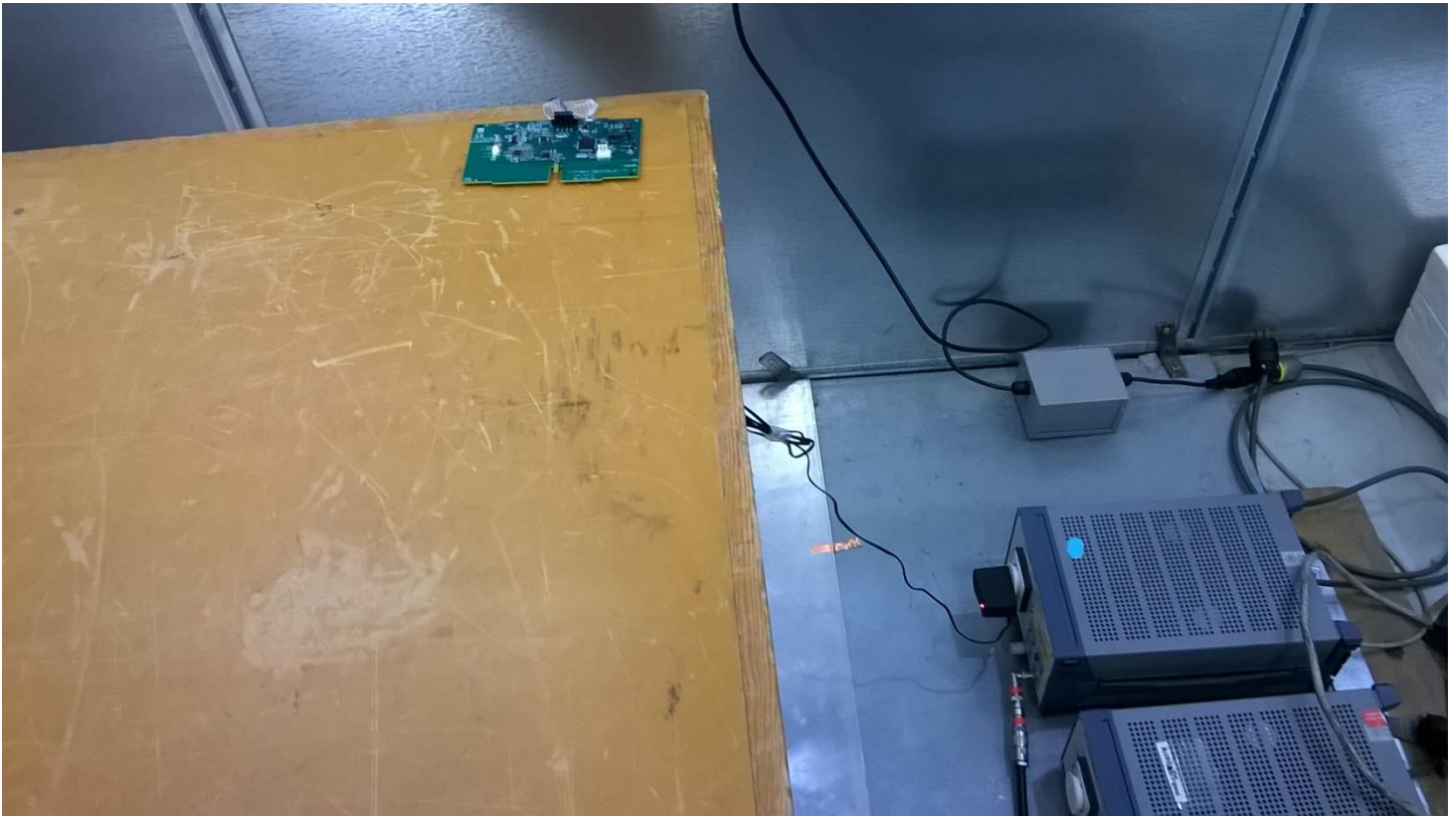
Figure 6 - Conducted Emissions Test Setup
