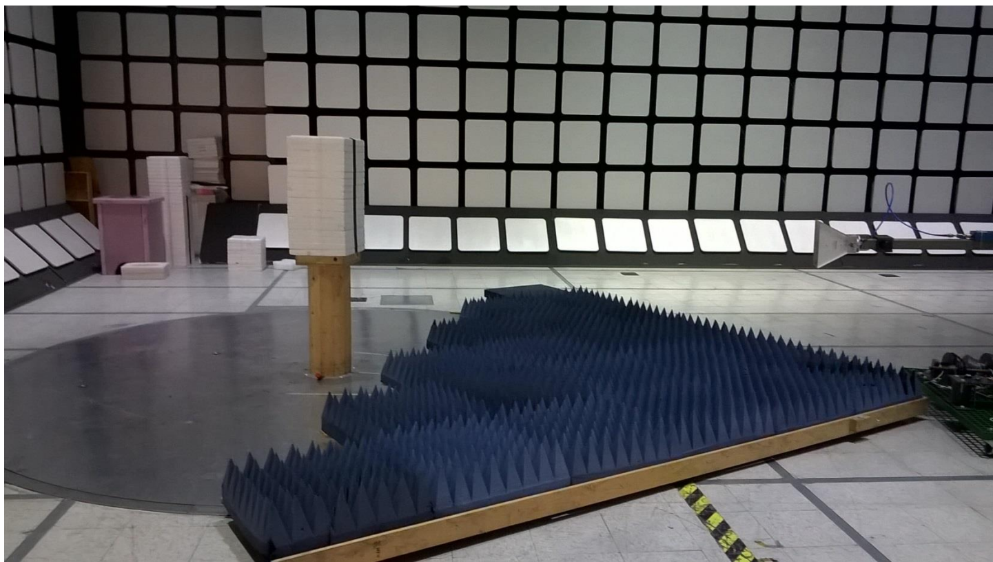
Figure 2 - Example test setup for radiated emissions, above 1 GHz.
