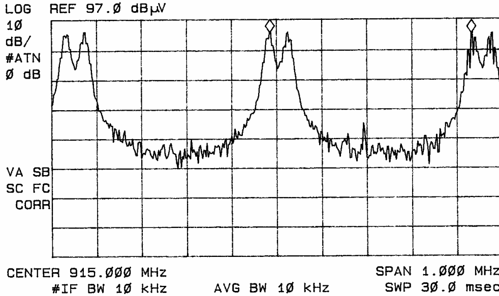
Figure nineteen Channel Spacing
