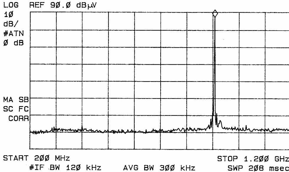
Figure seven General Radiated Emissions (Mounted Antenna).
