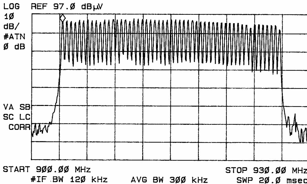
Figure fourteen Frequencies of operation (Mounted Antenna)
