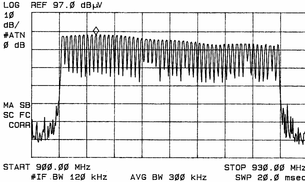
Figure thirteen Frequencies of operation (PCB Antenna)
