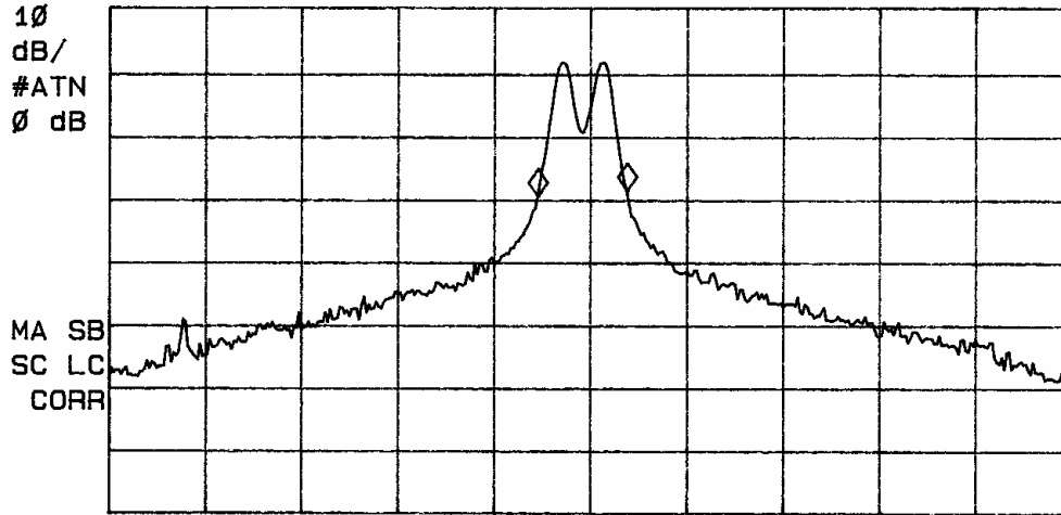
Figure seventeen Occupied Bandwidth high frequency
