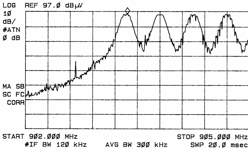
Figure twenty lower frequency band edge
