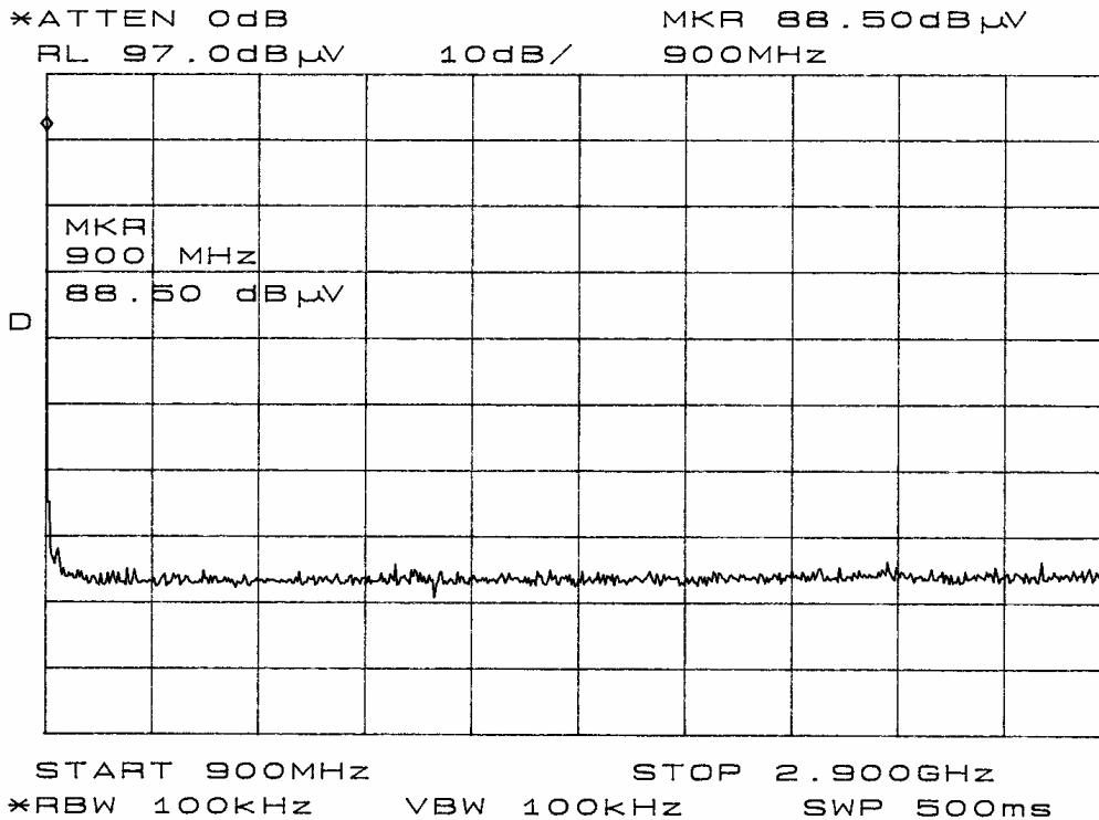
Figure eight General Radiated Emissions (Mounted Antenna).
