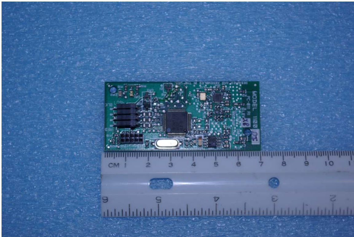
PCB Front PCB etched antenna
