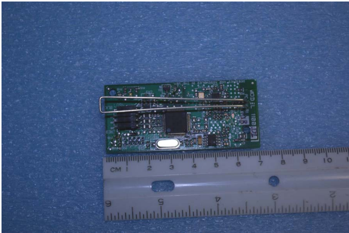
PCB Front PCB Factor mounted antenna
