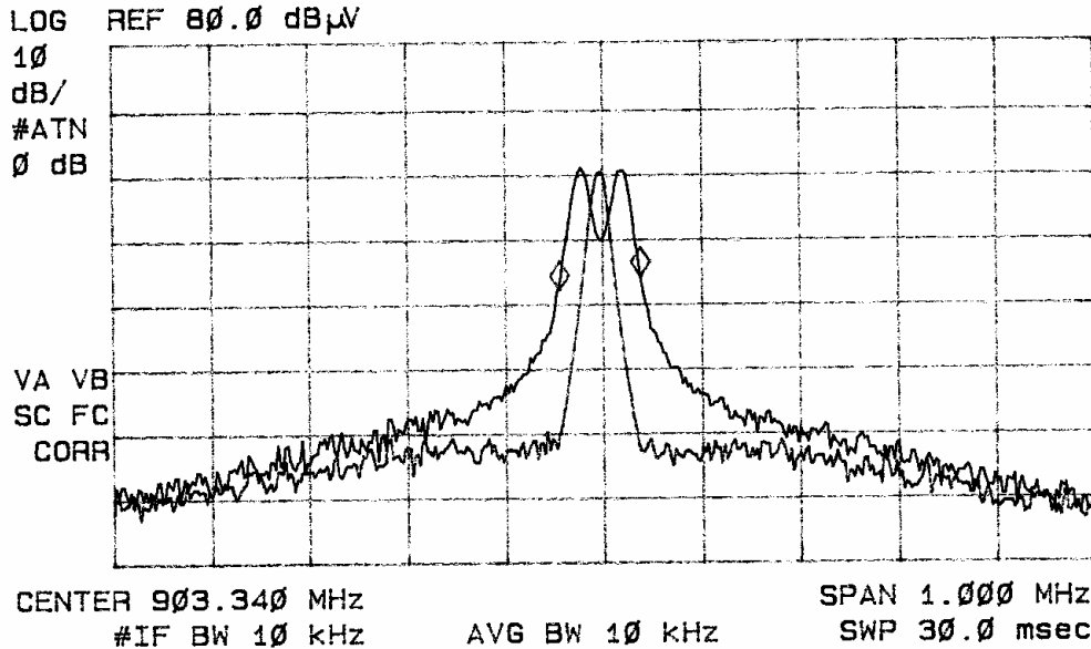
Figure fifteen Occupied Bandwidth low frequency (99% power).
