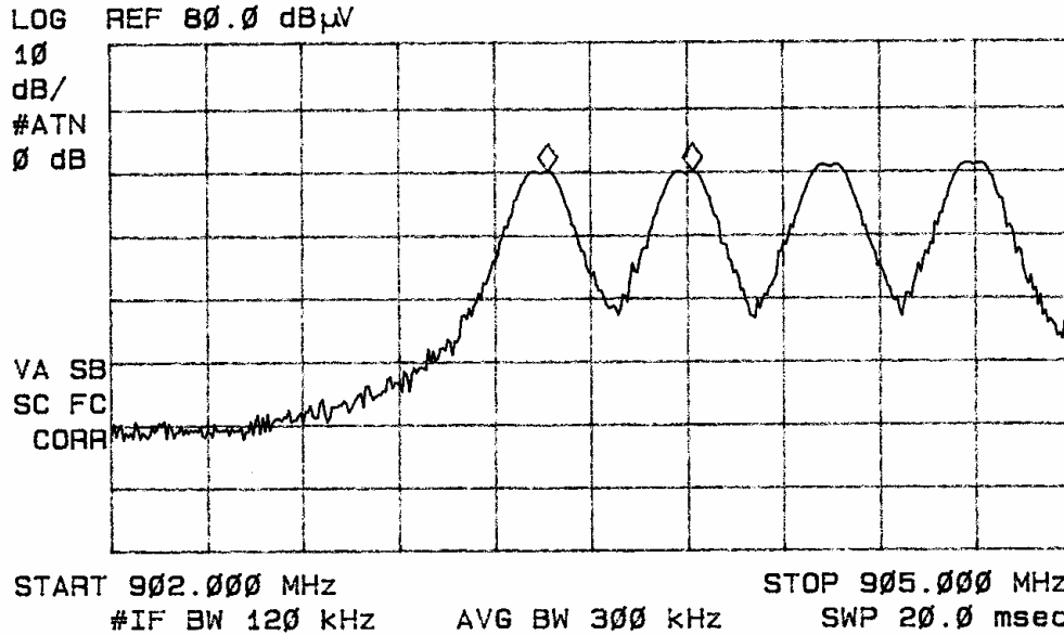
Figure nineteen Channel Spacing and low band edge.
