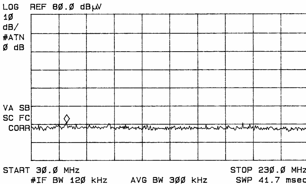
Figure eight Radiated Emissions taken at 1 meter in screen room (DC powered).
