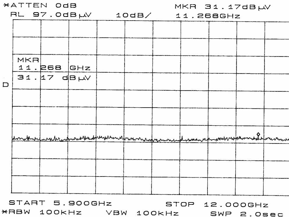
Figure twelve Radiated Emissions taken at 1 meter in screen room (DC powered).
