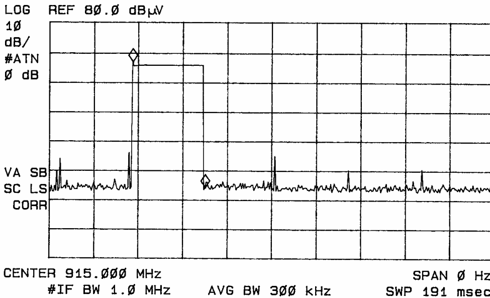
Figure eighteen Dwell Time on channel.
