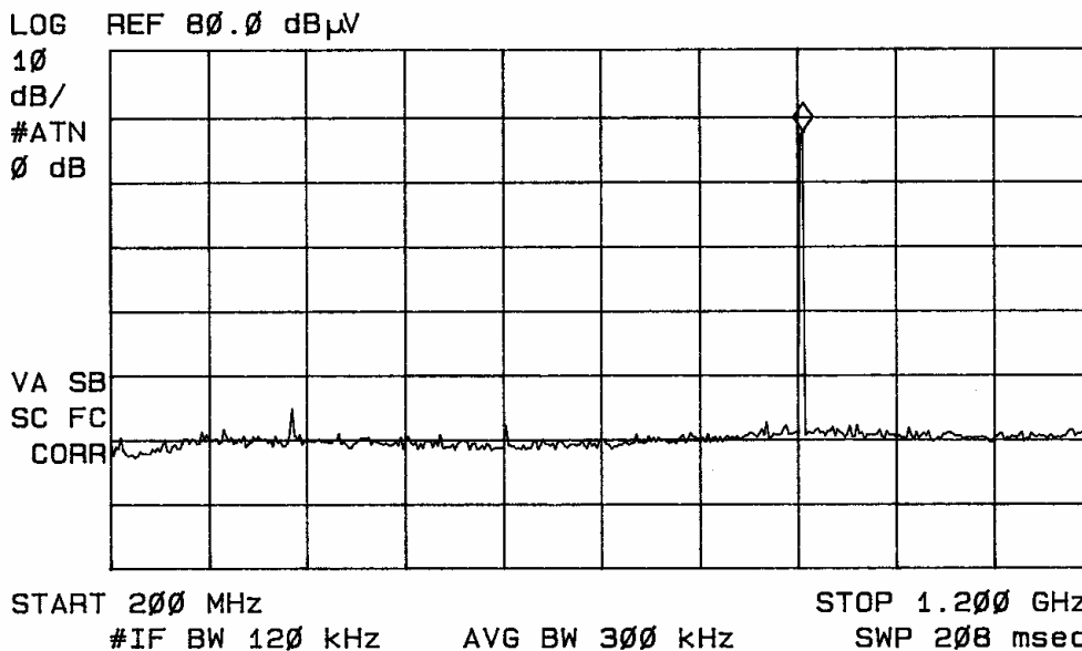
Figure four Radiated Emissions taken at 1 meter in screen room (AC powered).
