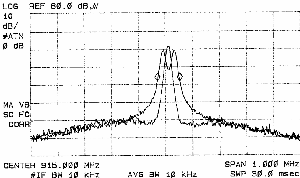
Figure sixteen Occupied Bandwidth middle frequency (99% power).
