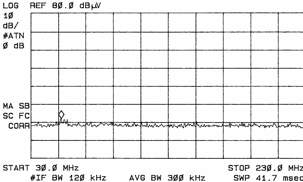
Figure three Radiated Emissions taken at 1 meter in screen room (AC powered).
