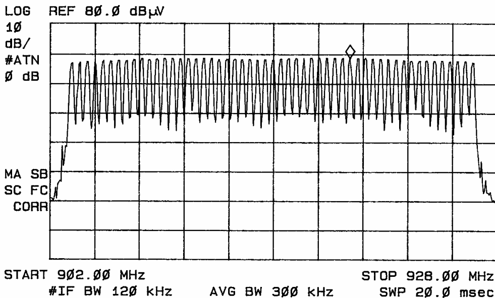
Figure fourteen Frequencies of operation.
