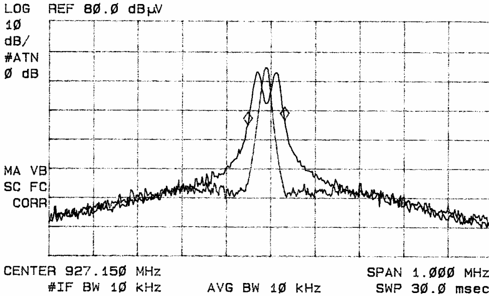
Figure seventeen Occupied Bandwidth high frequency (99% power).
