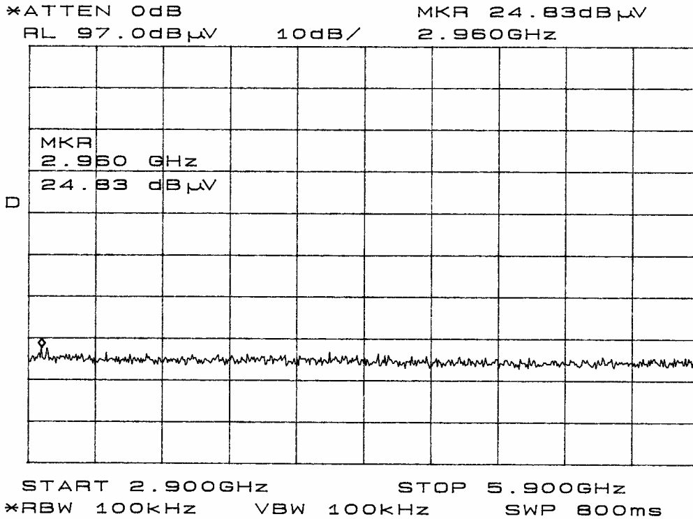
Figure eleven Radiated Emissions taken at 1 meter in screen room (DC powered).
