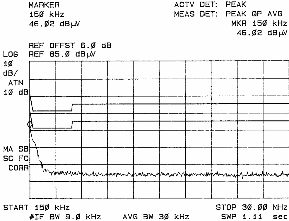
Figure one Conducted Emissions of Line 1 Taken in the Screen Room
