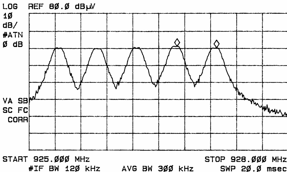
Figure twenty Channel Spacing and high band edge.
