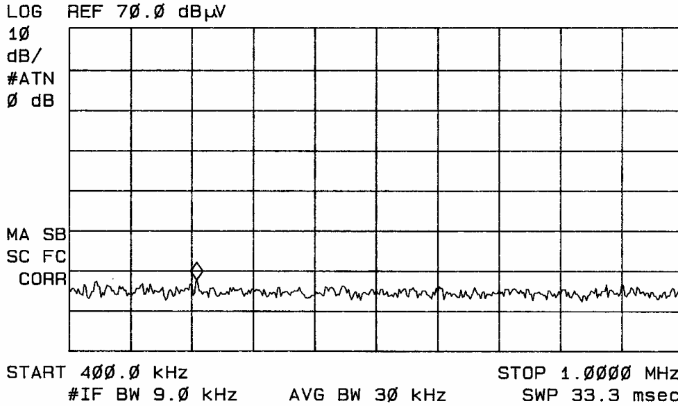
Figure six Radiated Emissions taken at 1 meter in screen room.
