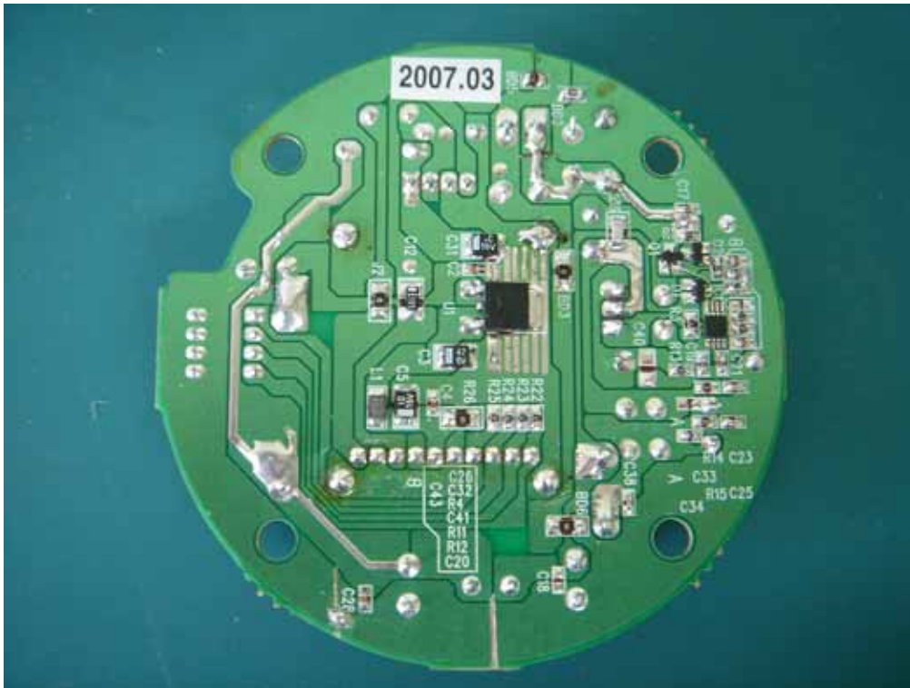
Soldered wire Antenna
