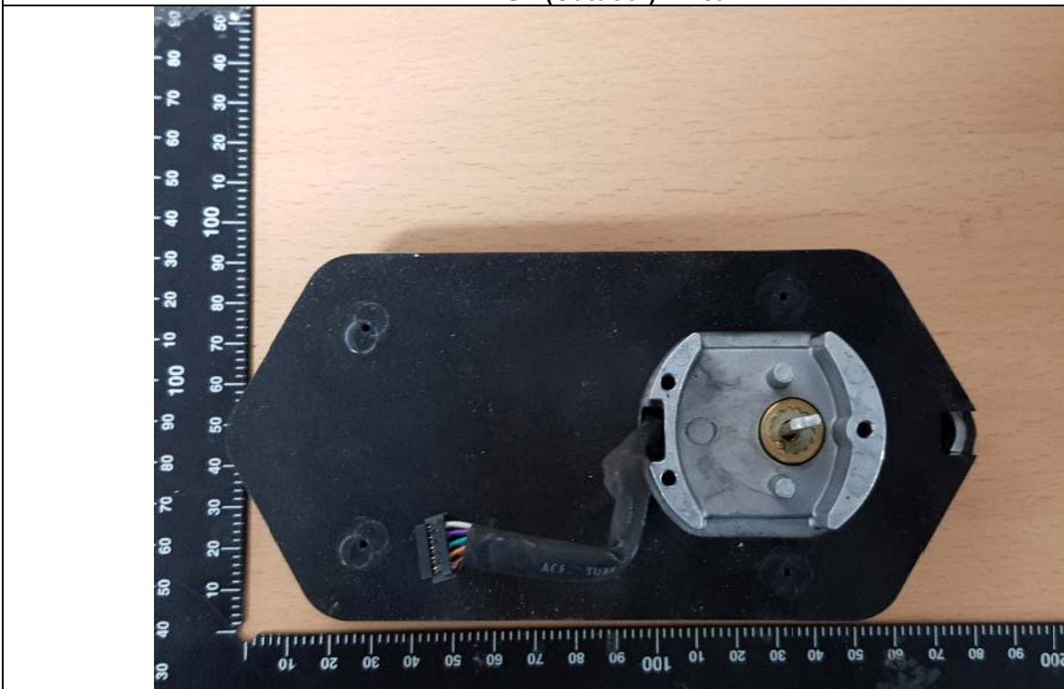
EUT (Outdoor) – Rear
