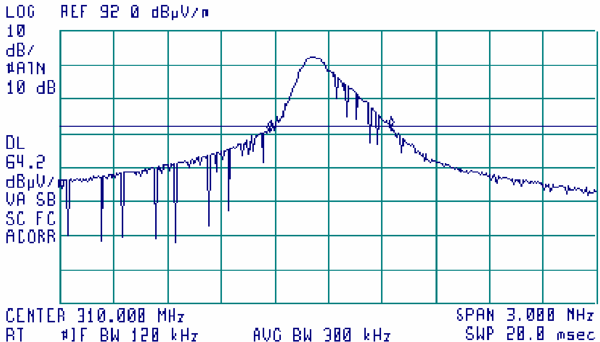
This chart shows a typical measured bandwidth signal.
