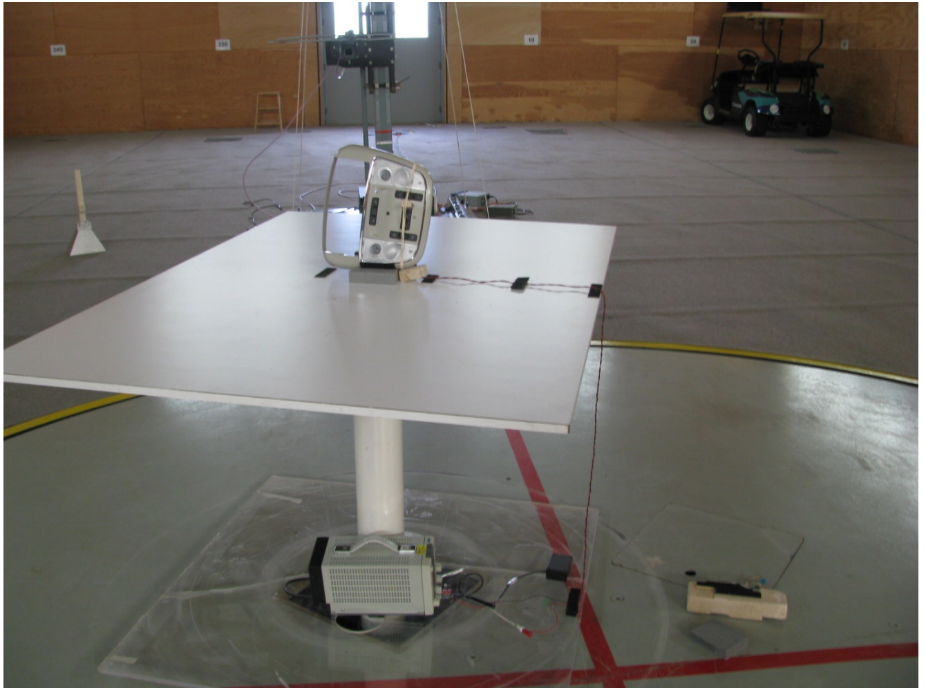
Test Setup Photograph 1: Device under test on a 1 x 1.5 meter non metallic table elevated 80 cm above a conducting ground plane. The harness providing power and ground runs to the long edge of the table and connects to a variable power supply underneath.
