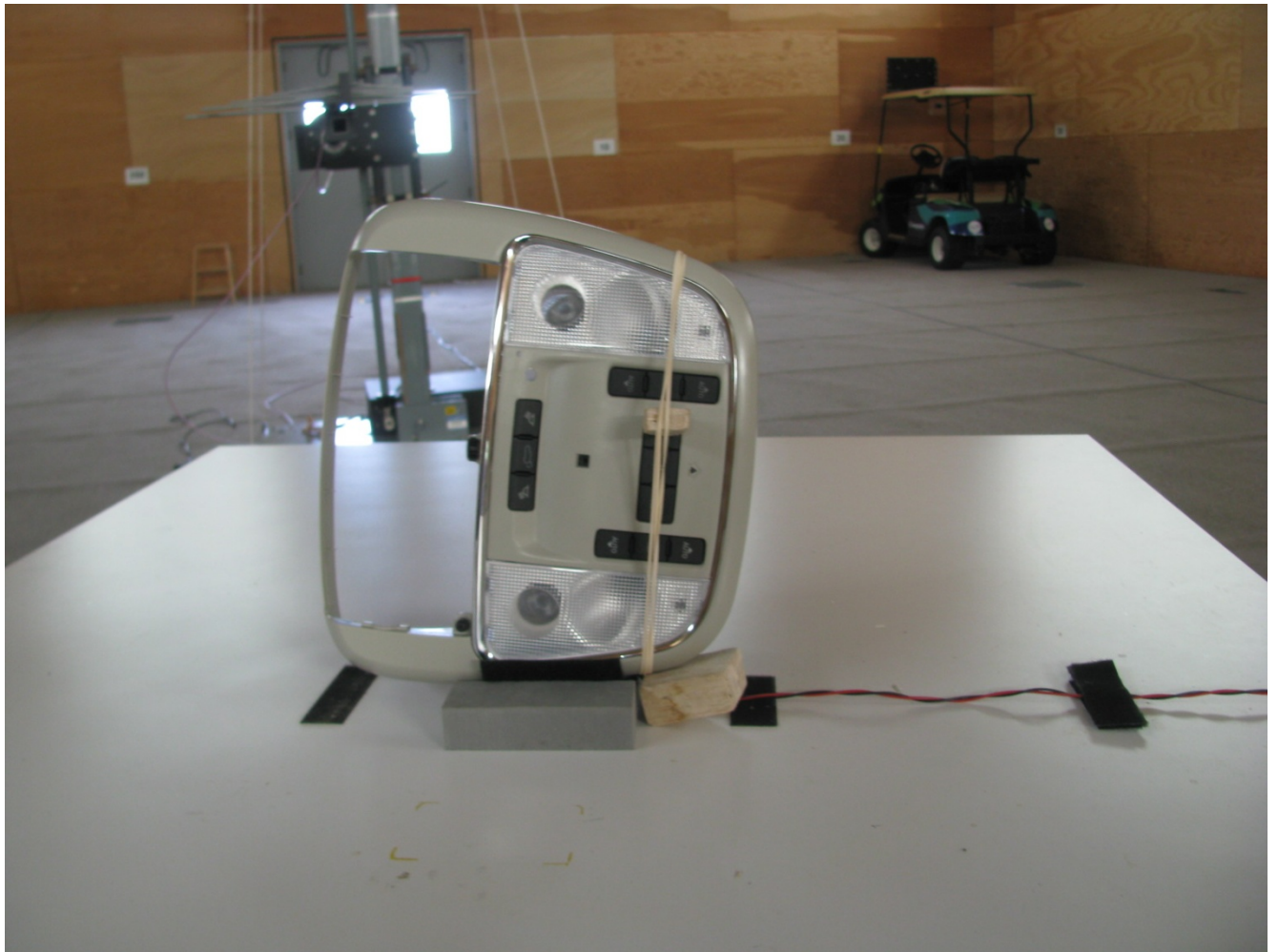
Test Setup Photograph 2: Device tested on its side. The button was depressed for constant transmit using a block and elastic band.
