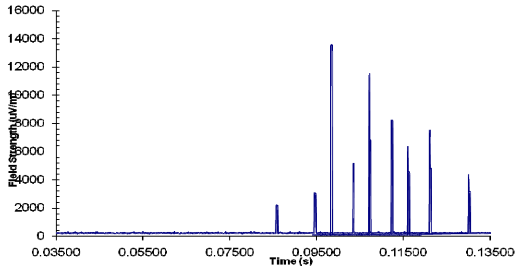
288 MHz, 30% Duty Cycle Tuning Pulse
