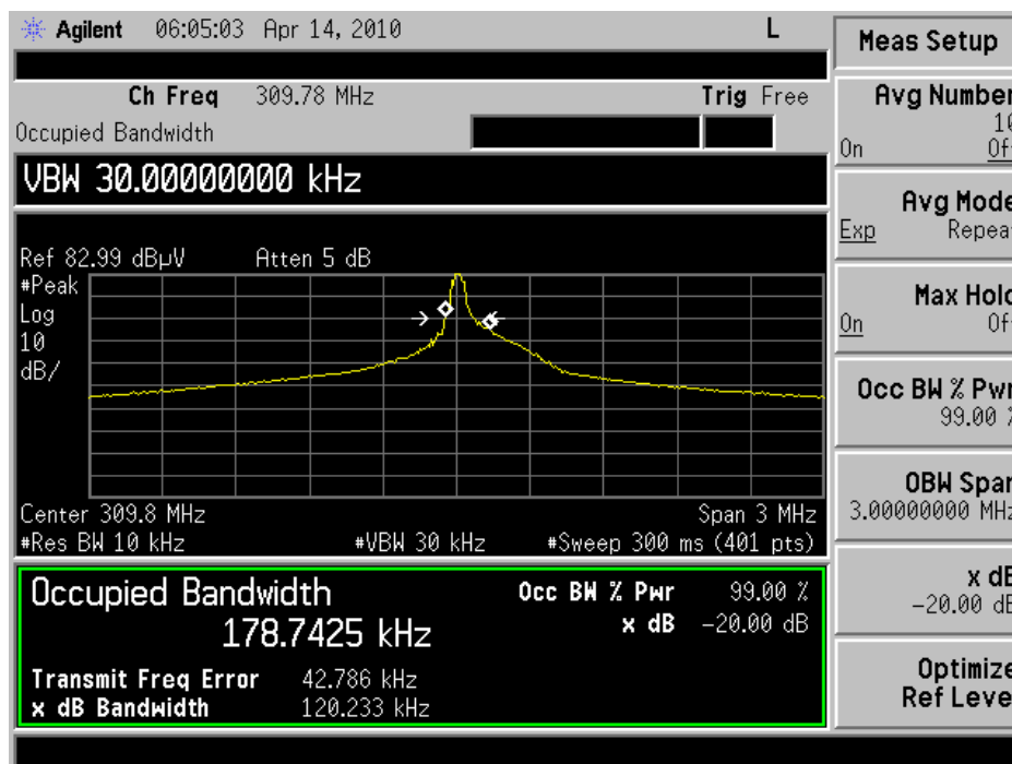
Measuring Occupied Bandwidth at -20dB points
