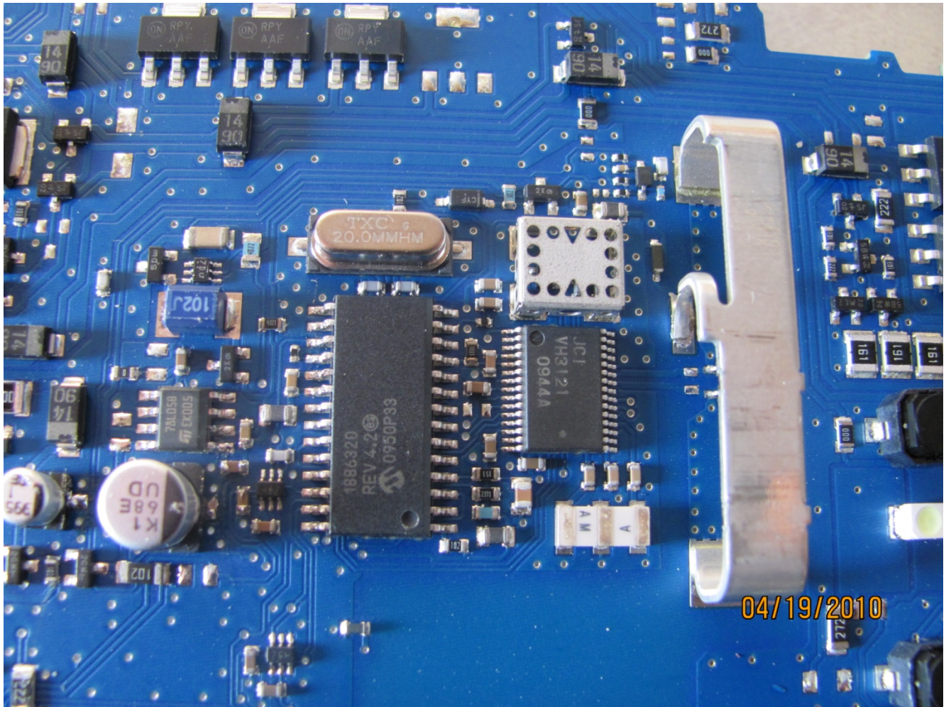
Internal Photograph 6: Detail view of RF portion of circuit board with the antenna on the right side of photograph.
