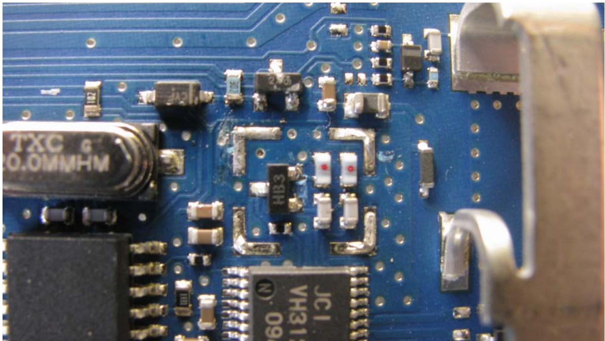
Internal Photograph 7: Detail view of RF circuit with shield removed.
