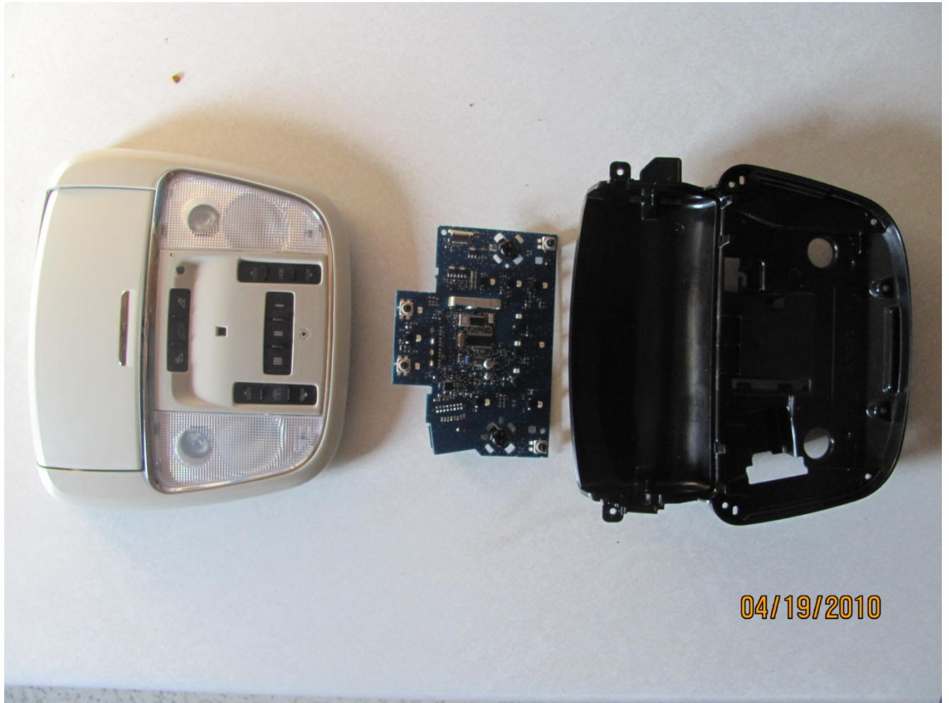
Internal Photograph 3: Disassembled view, front side of components.
