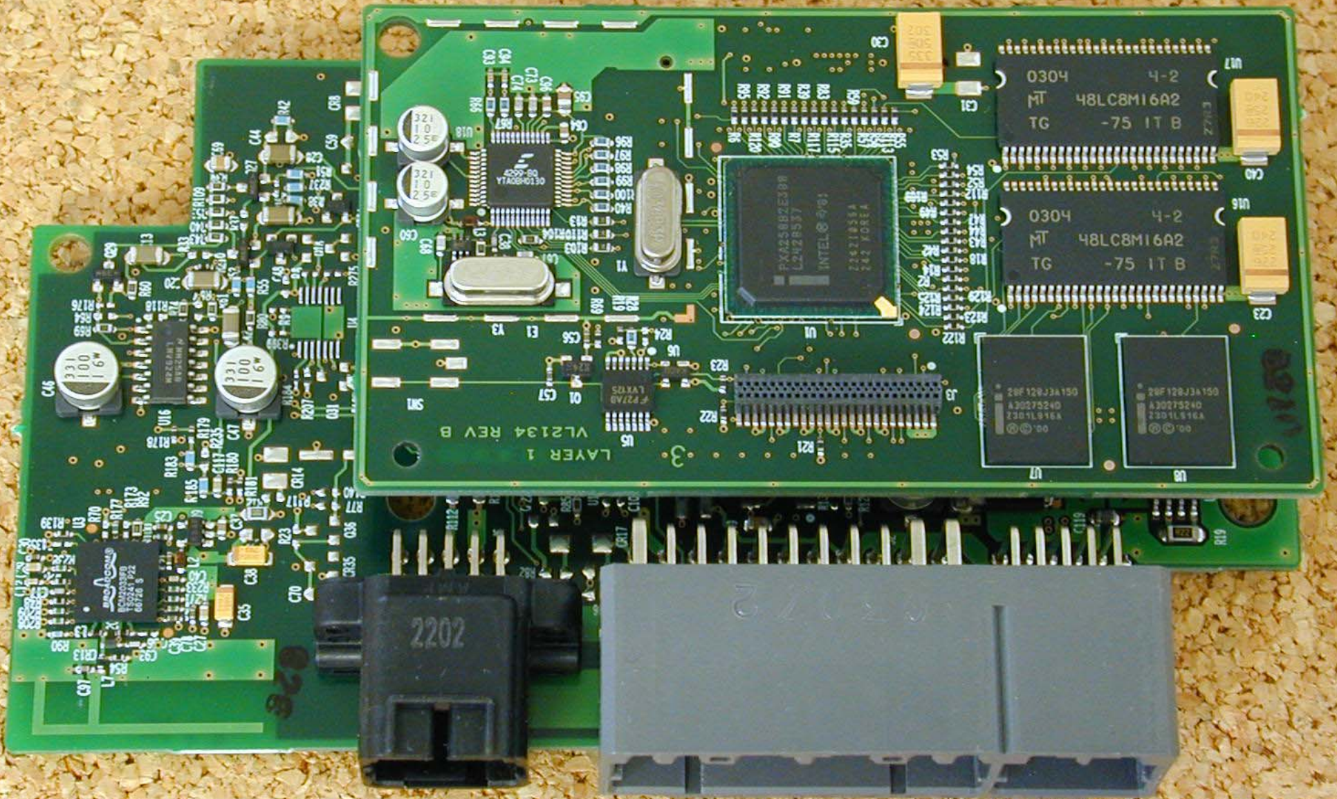
Module 05064022AE PCB (top)
