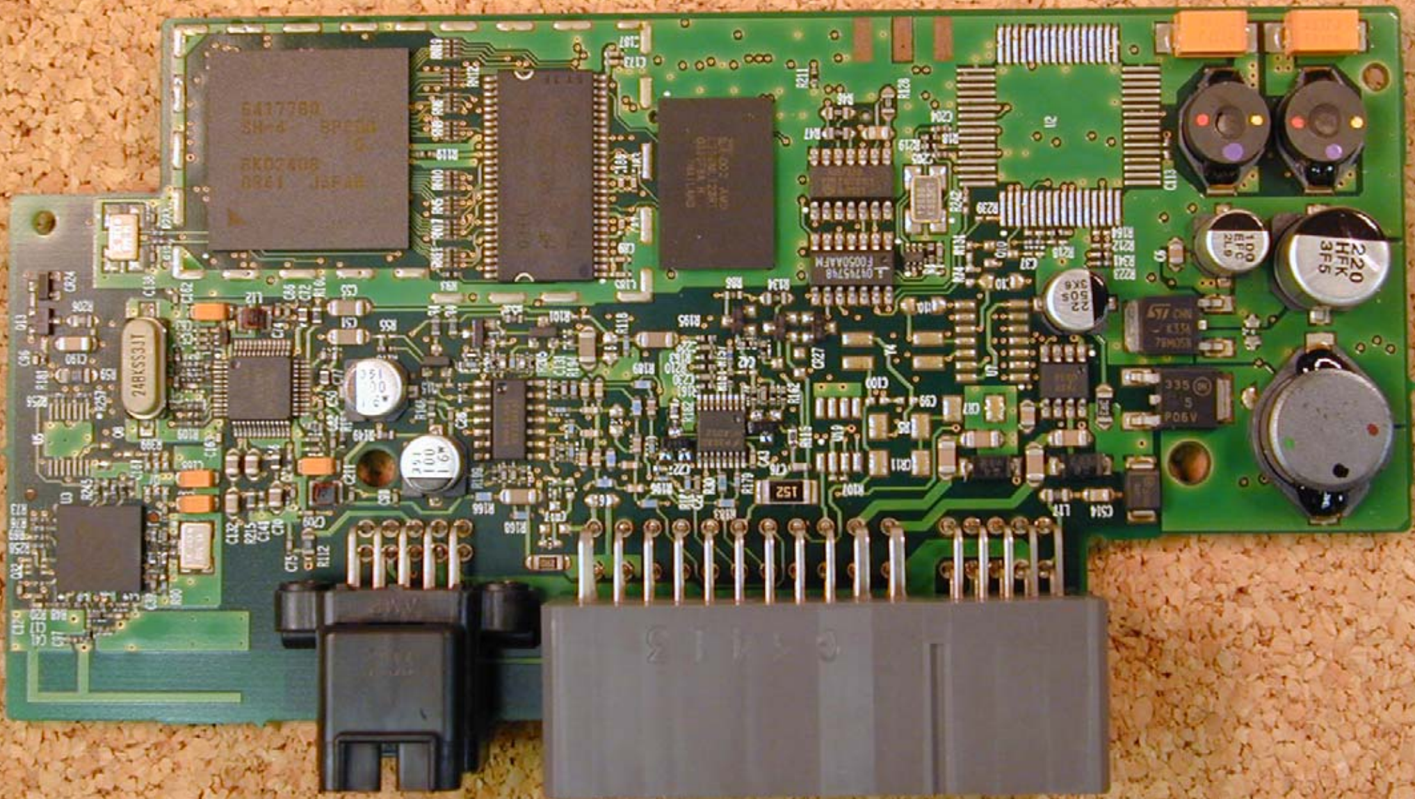
PCB (J1850 Diff) top
