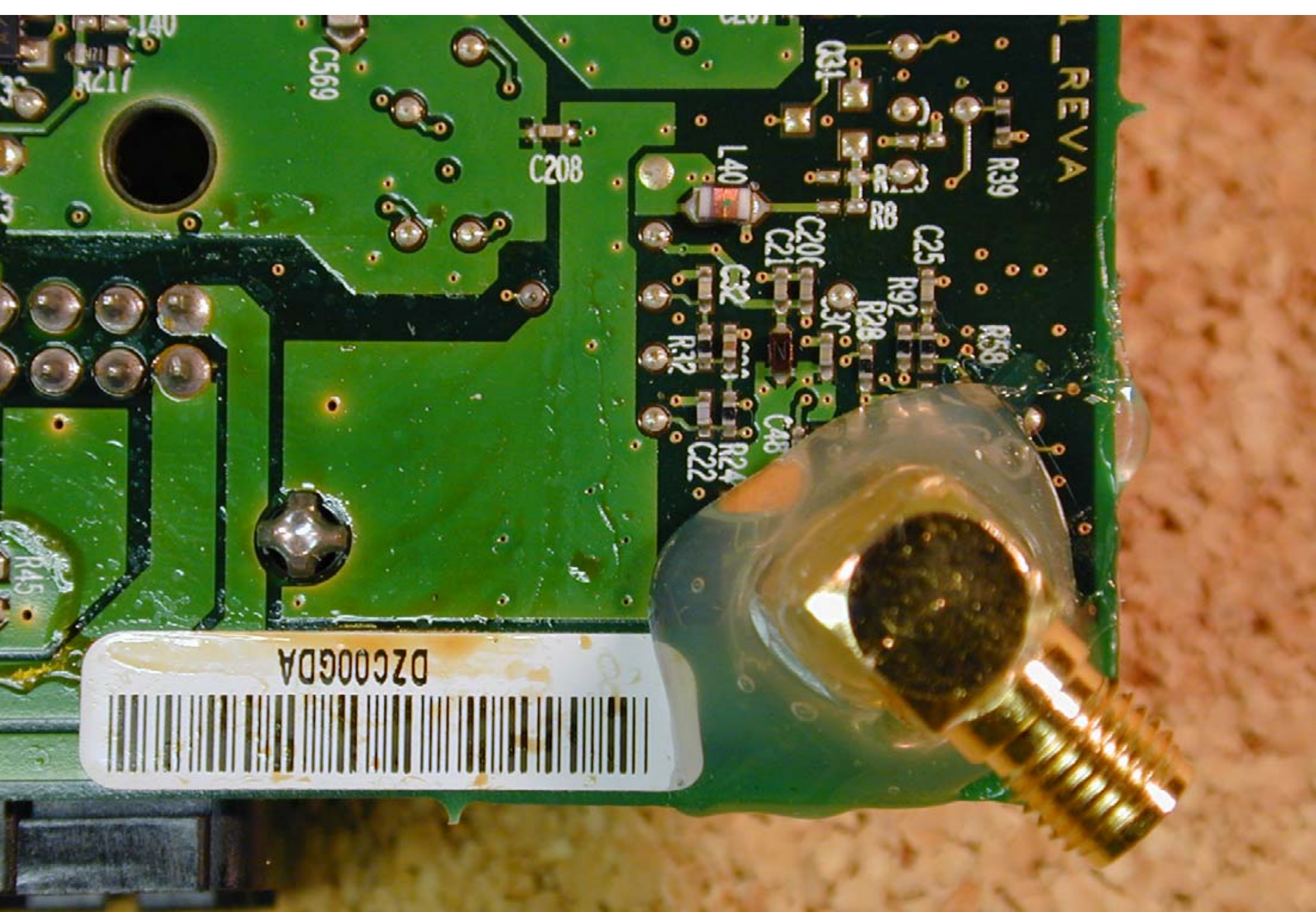
PCB (J1850 Diff) Modified for Conducted (bottom)
