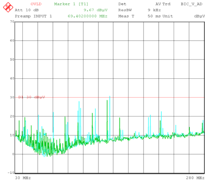
Title: DUT F2 / G6-7 w/ HL TX on Ch.3 Date: 4.AUG.2004 19:23:43
