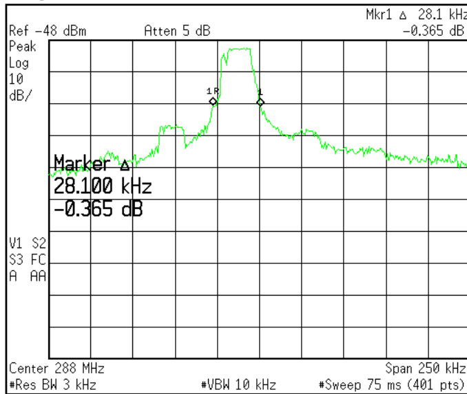
Measuring Occupied Bandwidth
