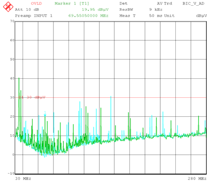
Title: DUT F2 / G6-7 w/ HL TX on Ch.3 Date: 4.AUG.2004 19:18:25
