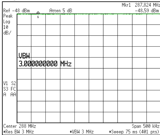
Determining Reference level.
