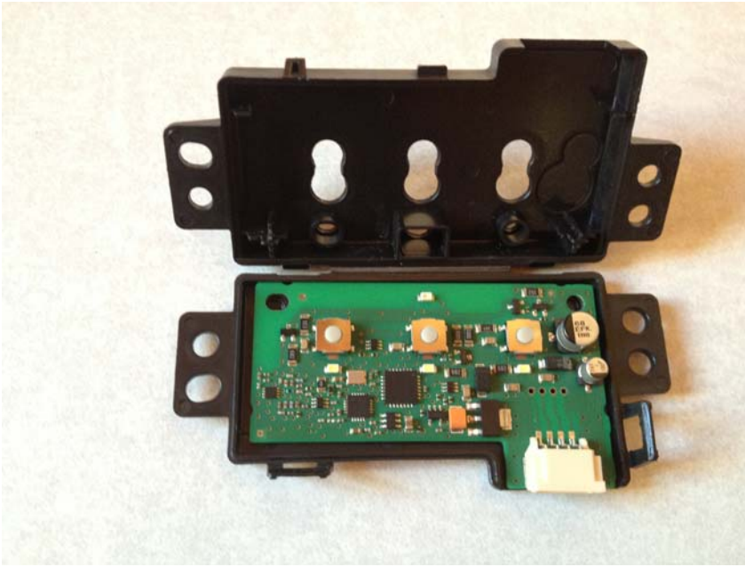
Homelink inside housing
