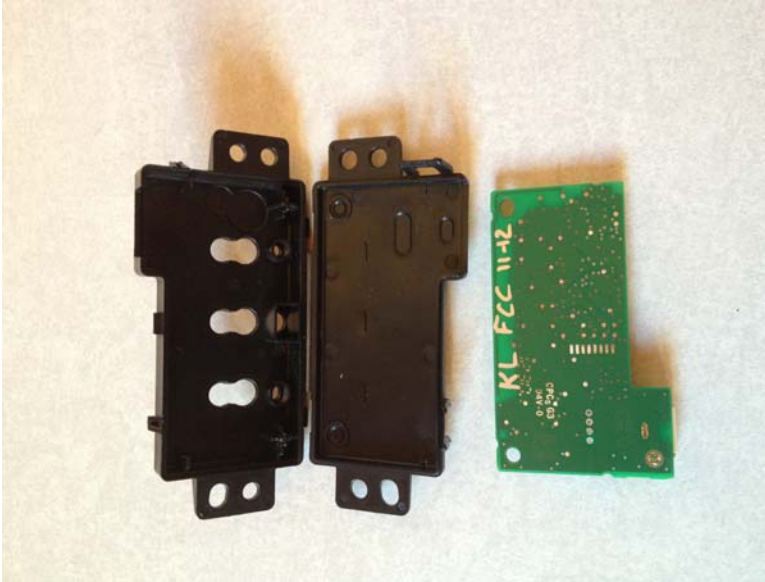
Front View with HL apart from Assembly Unit
