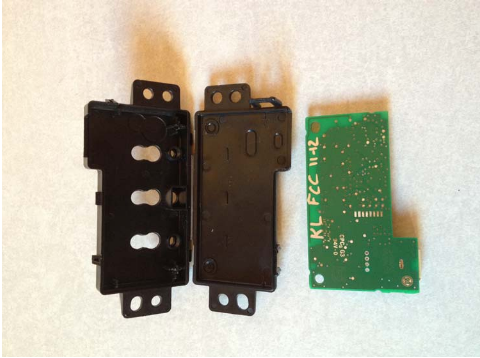
8.2 Housing & PCB Board Internal View
