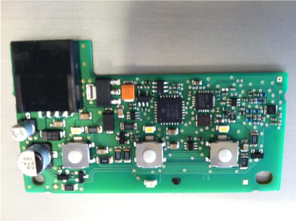
Internal View- Front
