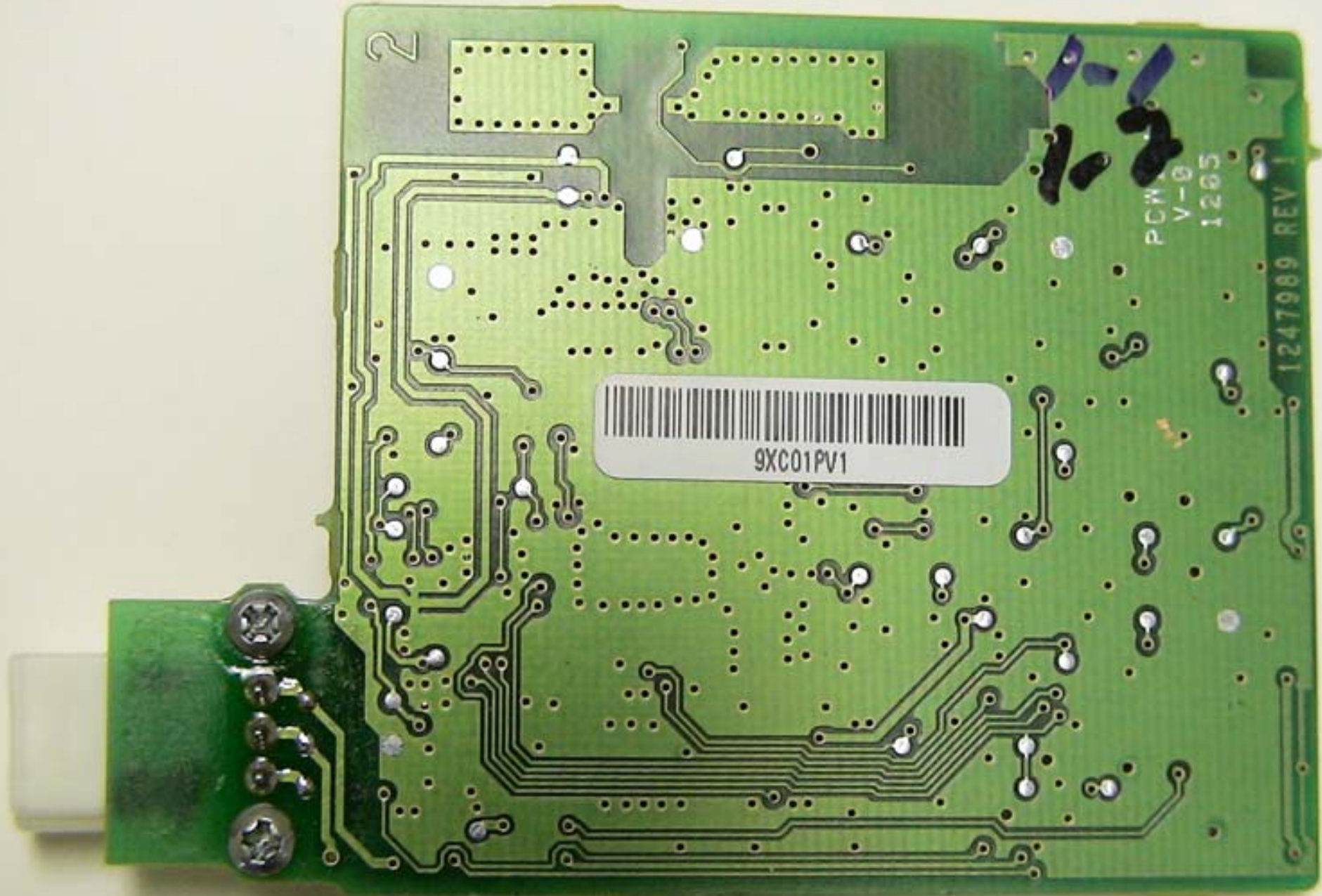
PCB (bottom)
