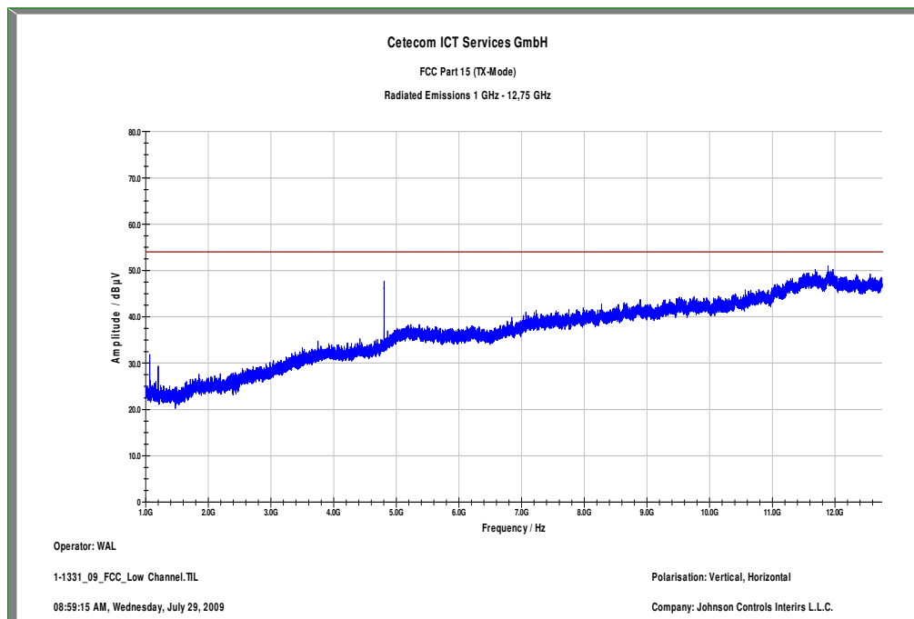
Signal suppressed with a 2.4 GHz band-reject filter
