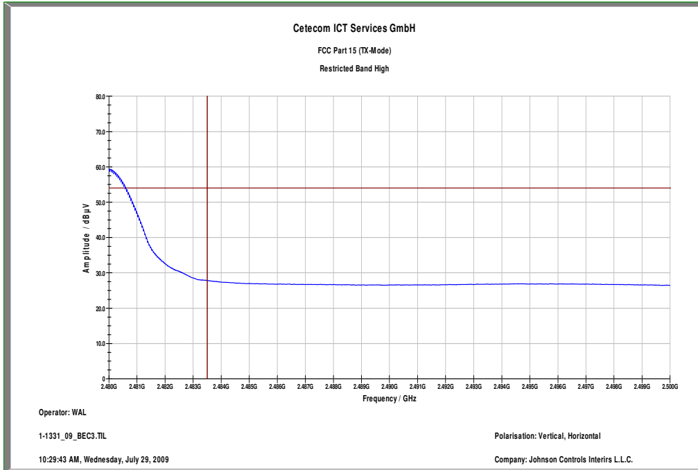
Plot 5: Band edge compliance at the highest channel with far away emissions
