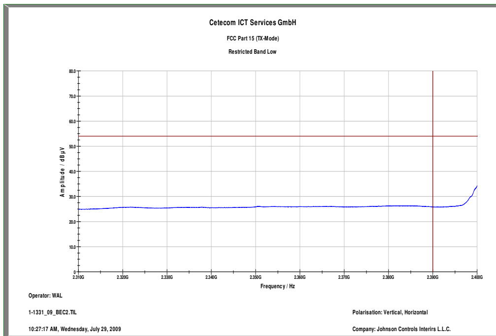
Plot 4: Band edge compliance at the lowest channel with far away emissions
