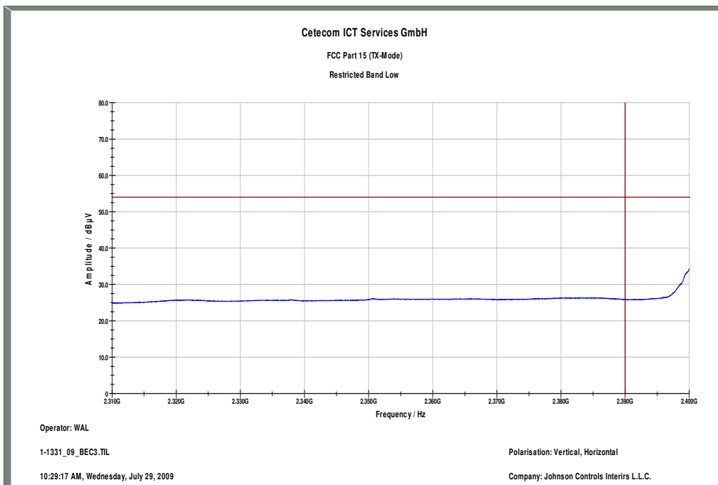
Plot 6: Band edge compliance at the lowest channel with far away emissions
