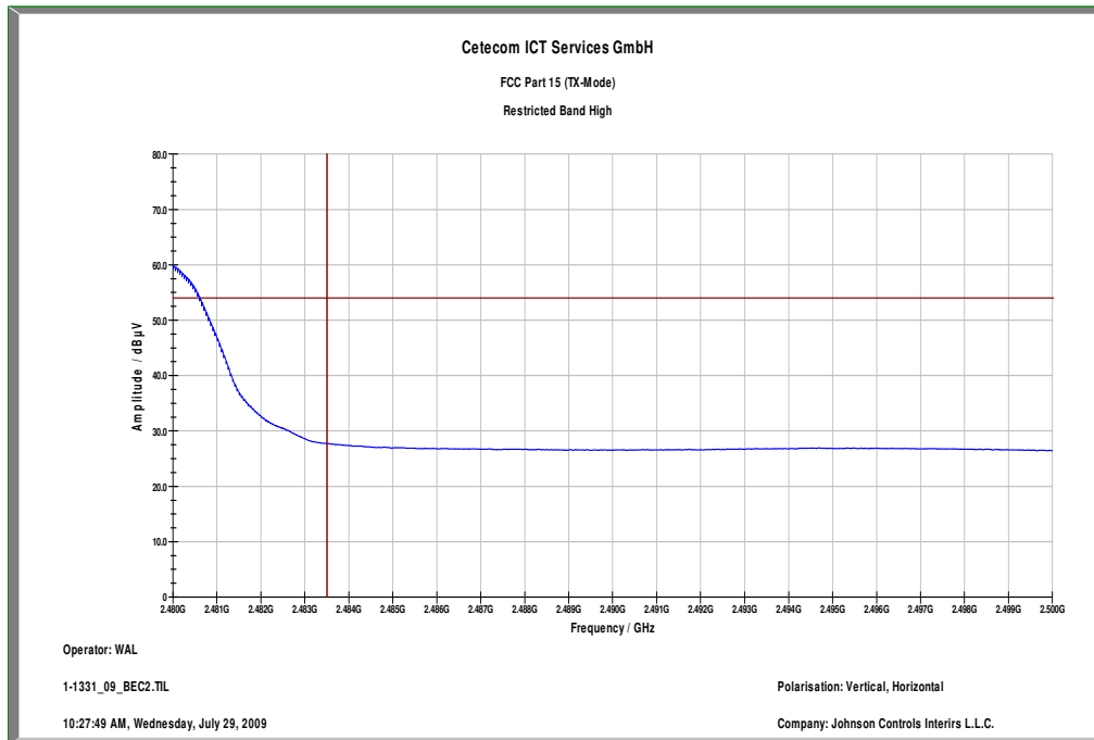
Plot 3: Band edge compliance at the highest channel with far away emissions
