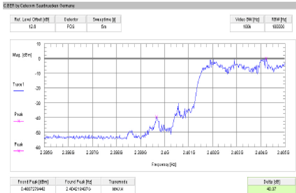
Plot 5: Lower band edge – hopping on / Pi/4 DQPSK (conducted)
