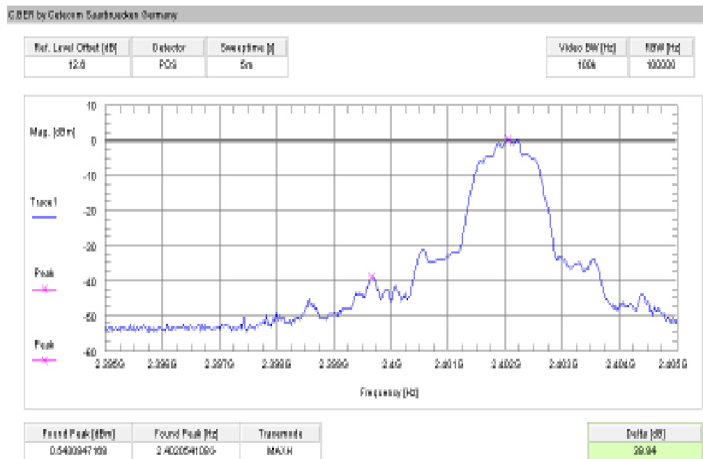
Plot 7: Lower band edge – hopping off / Pi/4 DQPSK (conducted)
