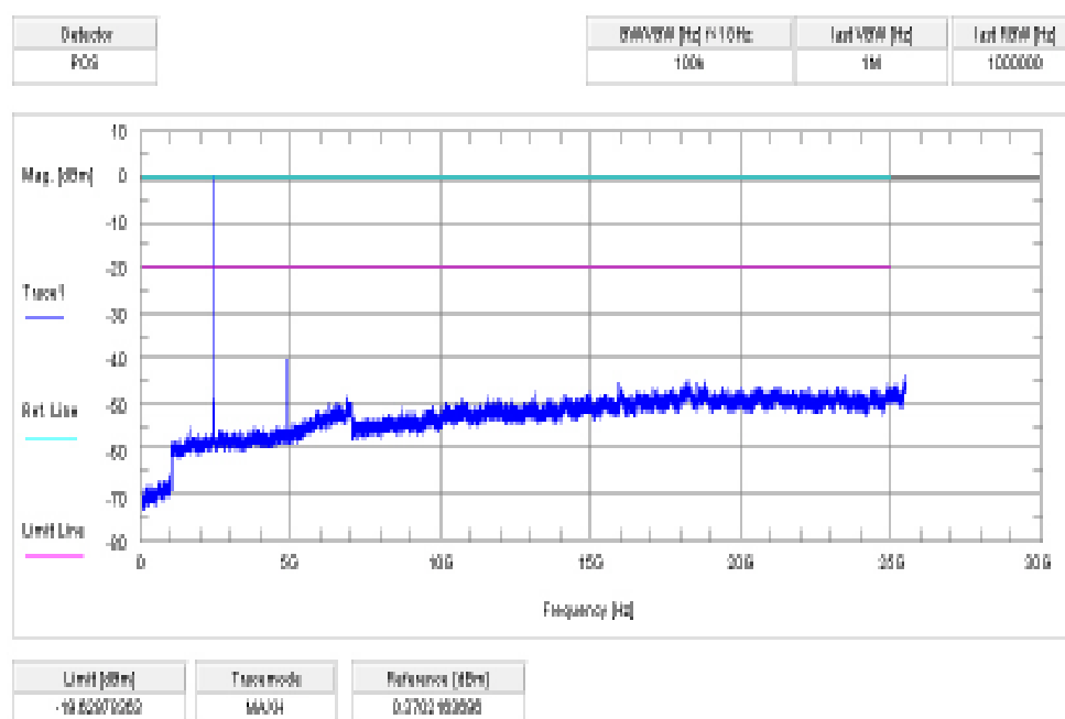
Plot 8: Channel 00 / 8DPSK
