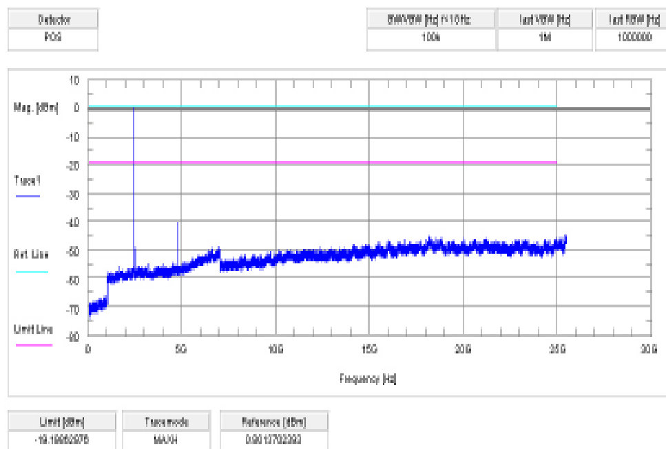
Plot 7: Channel 00 / 8DPSK
