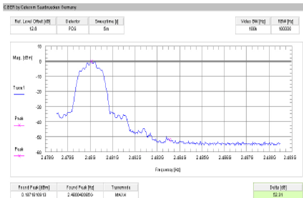
Plot 8: Upper band edge – hopping off / Pi/4 DQPSK (conducted)
