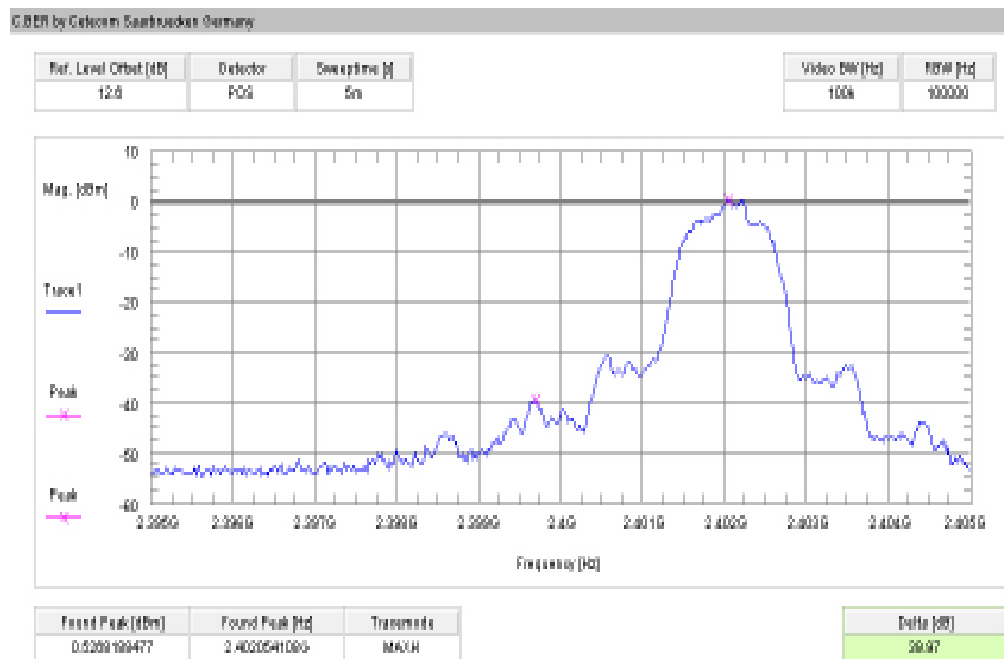
Plot 11: Lower band edge – hopping off / 8DPSK (conducted)
