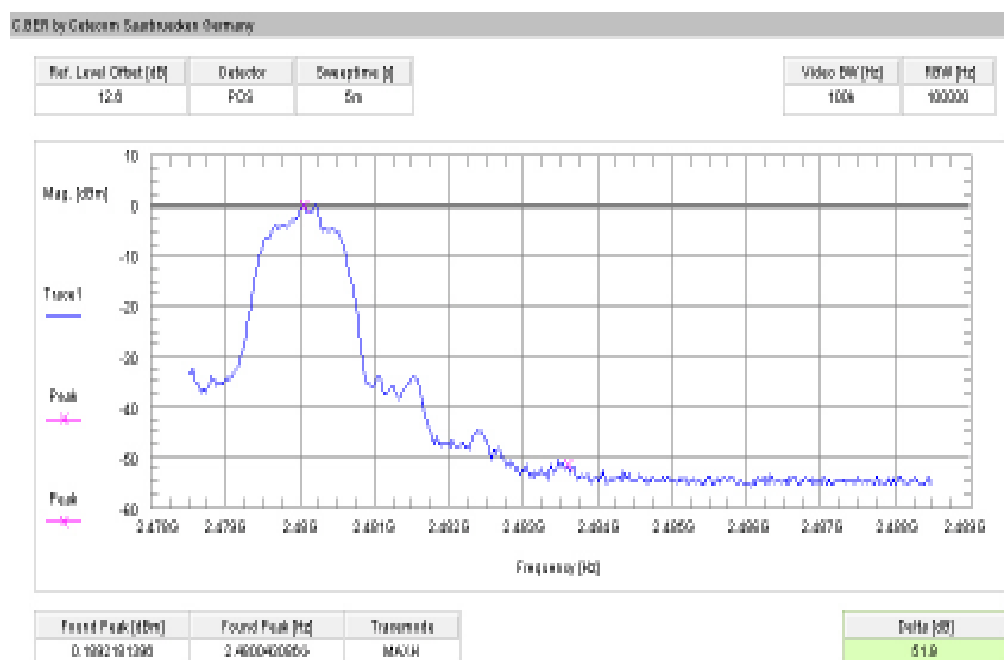
Plot 12: Upper band edge – hopping off / 8DPSK (conducted)
