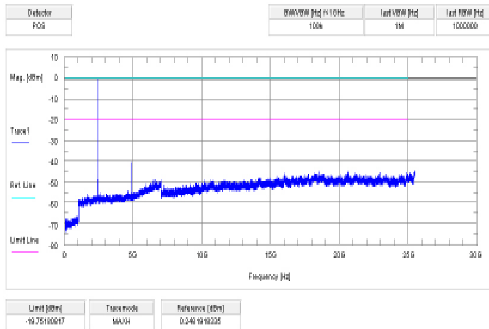
Plot 5: Channel 39 / Pi/4 DQPSK
