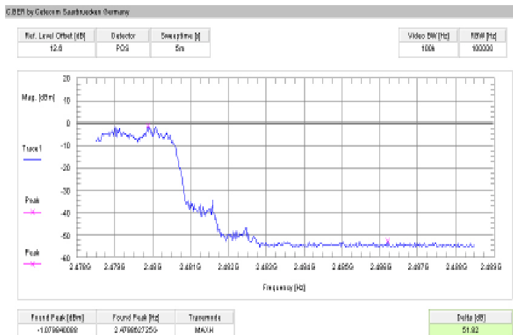
Plot 6: Upper band edge – hopping on / Pi/4 DQPSK (conducted)
