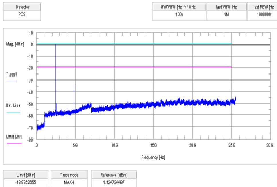
Plot 1: Channel 00 / GFSK
