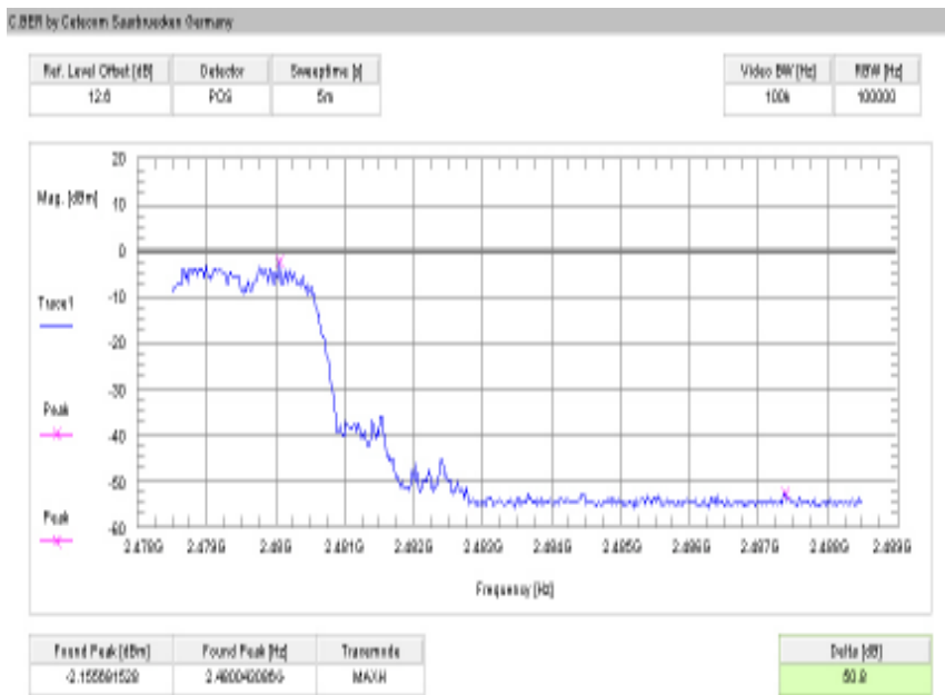
Plot 10: Upper band edge – hopping on / 8DPSK (conducted)
