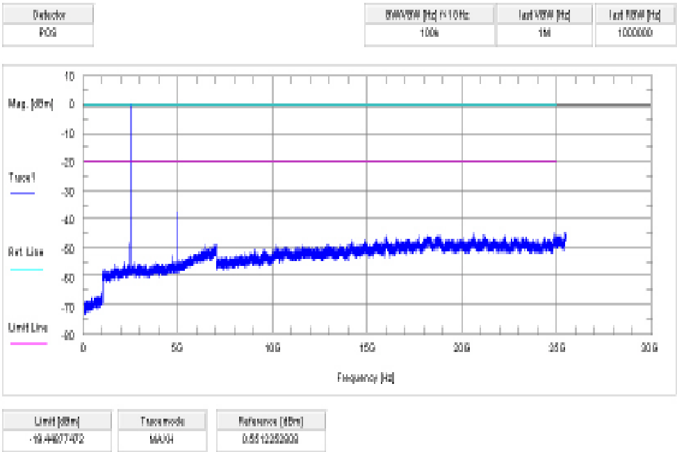
Plot 9: Channel 00 / 8DPSK
