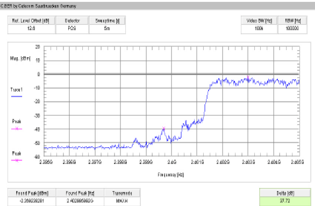
Plot 9: Lower band edge – hopping on / 8DPSK (conducted)
