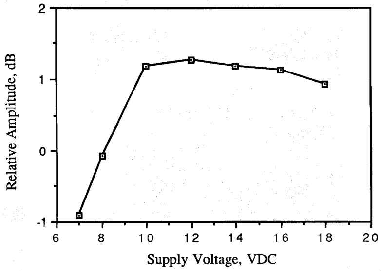
Figure 6.4. Relative emission vs. supply voltage. (310 MHz, CW)
