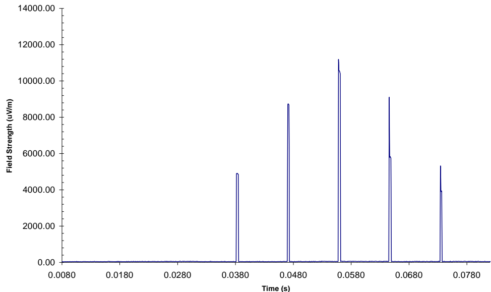
288 MHz, 30% Duty Cycle Tuning Pulse
