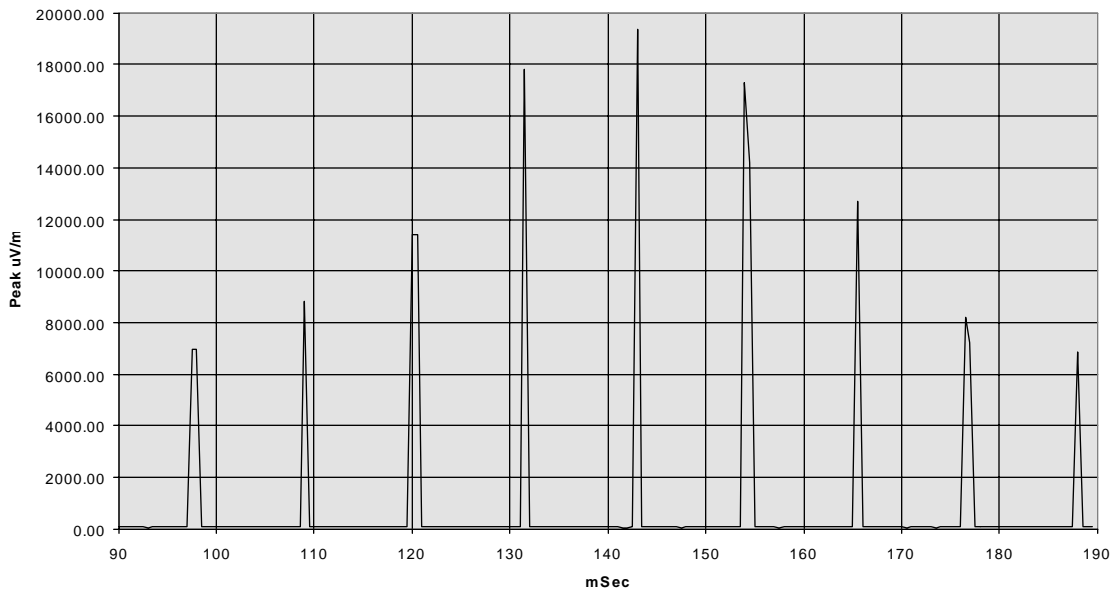
Fine Tune Pulses, 310MHz fundamental Linear Scale
