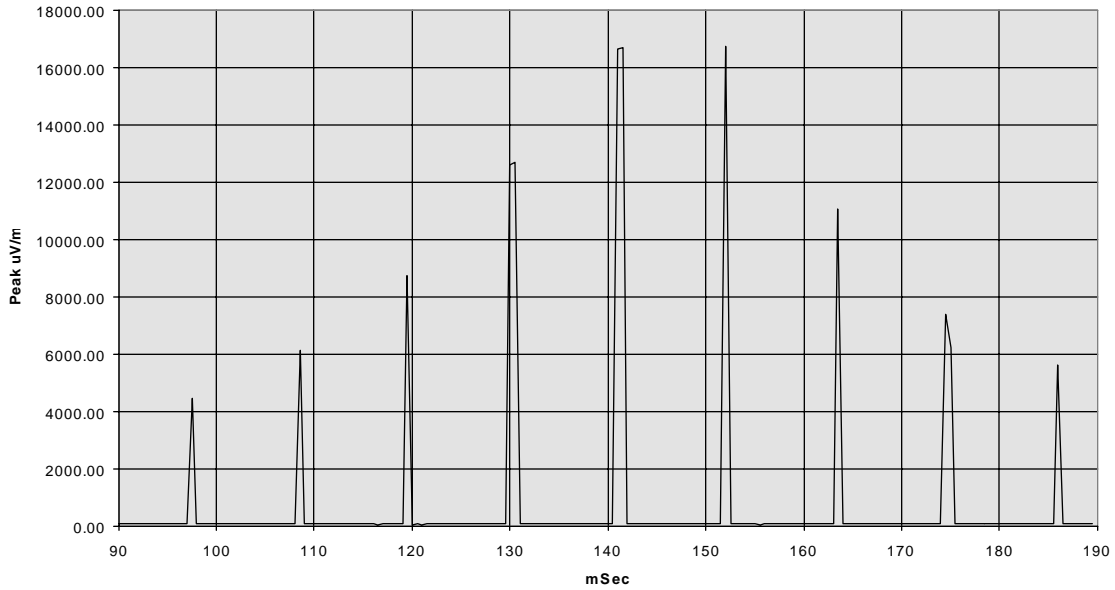
Fine Tune Pulses, 288MHz fundamental Linear Scale
