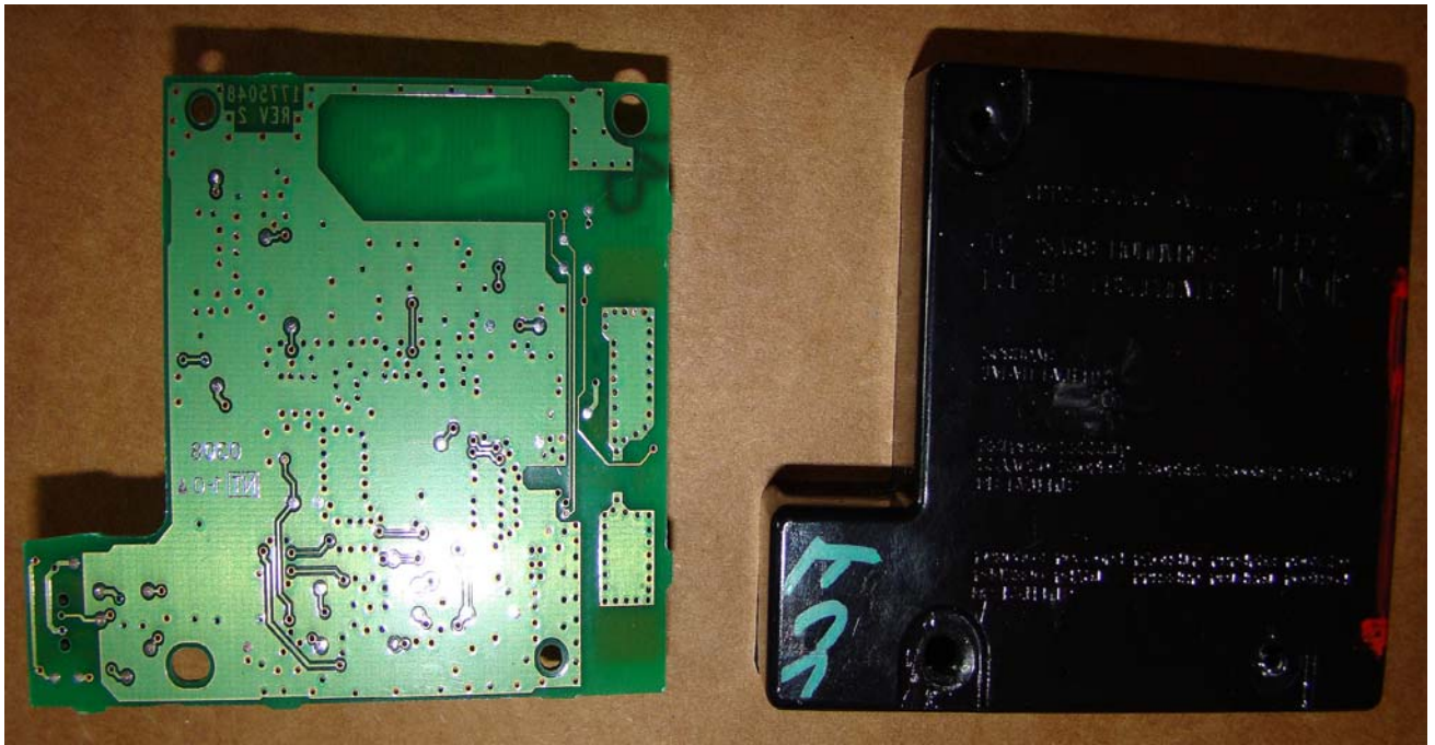
Internal View- Rear PCB side
