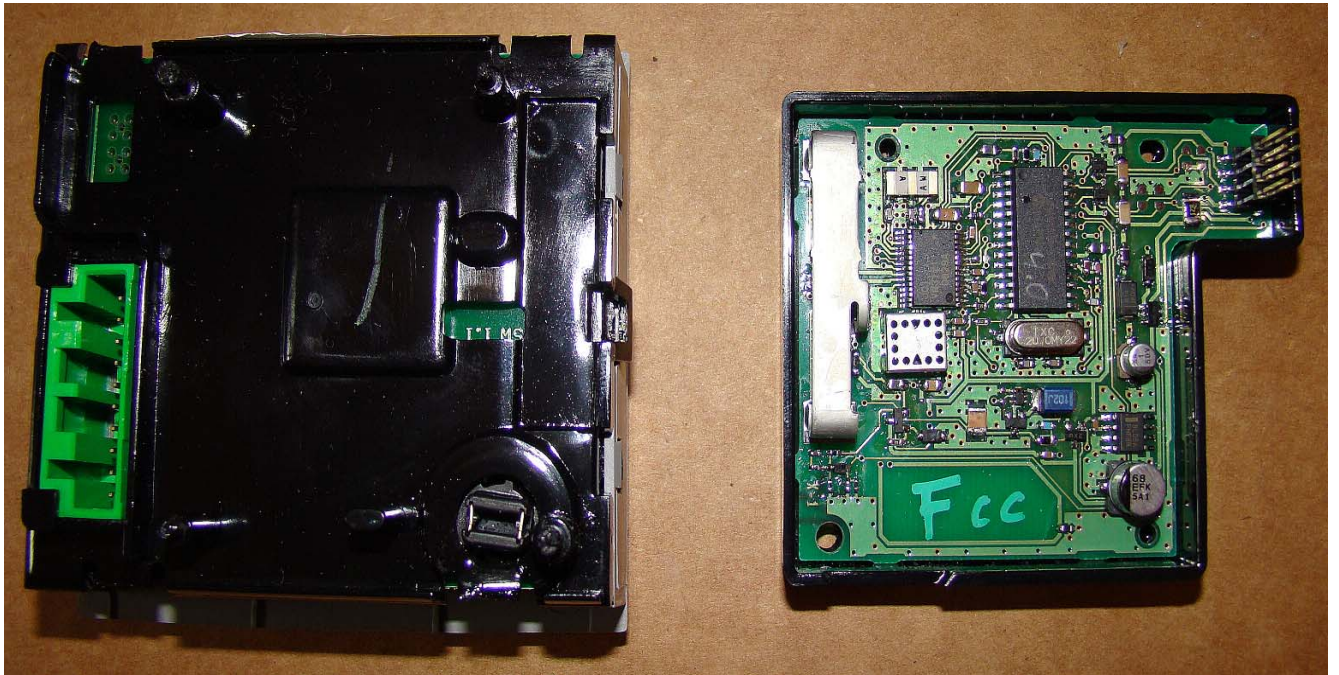
Unit Disassembled View
