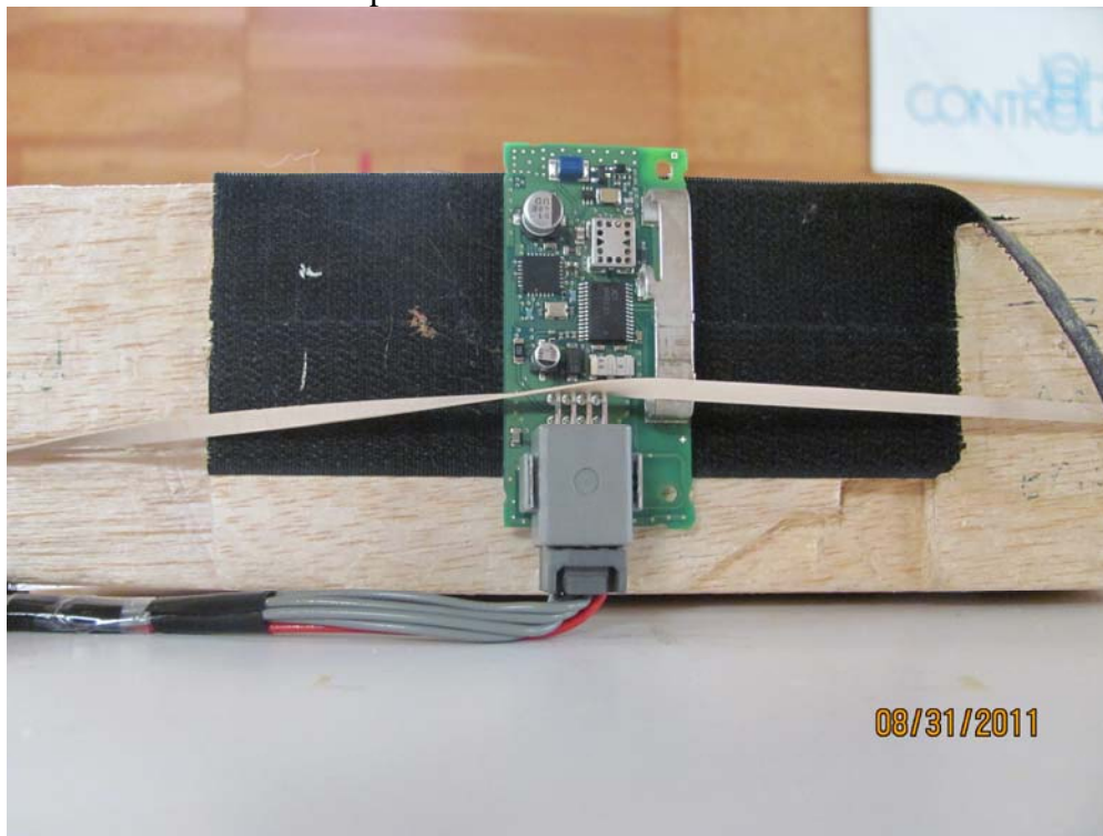
Test Set Up End
