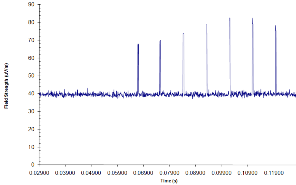
288 MHz, 30% Duty Cycle Tuning Pulse
