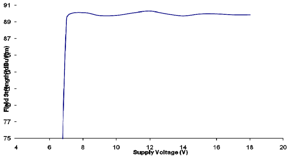
Output Field Strength vs. Supply Voltage
