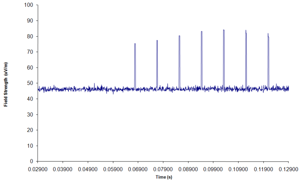
310 MHz, 30 % Duty Cycle Tuning Pulse
