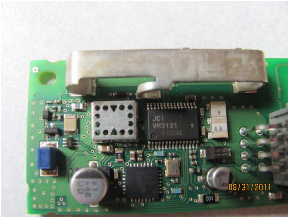
Close-up of Homelink RF
