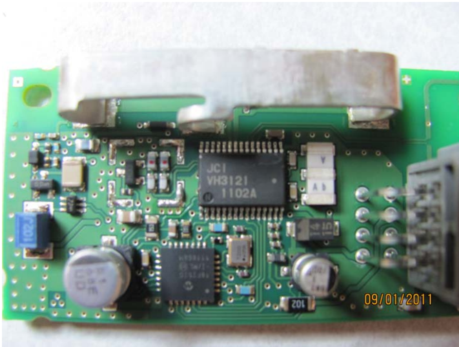
Close-up of Homelink RF shield removed
