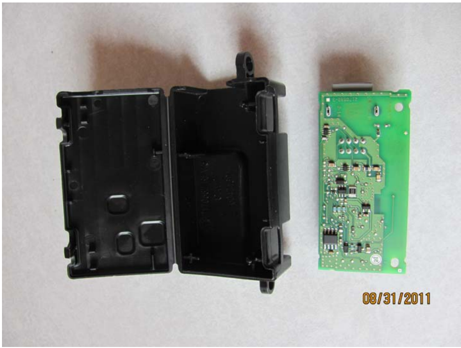
Rear View with HL apart from Assembly Unite
