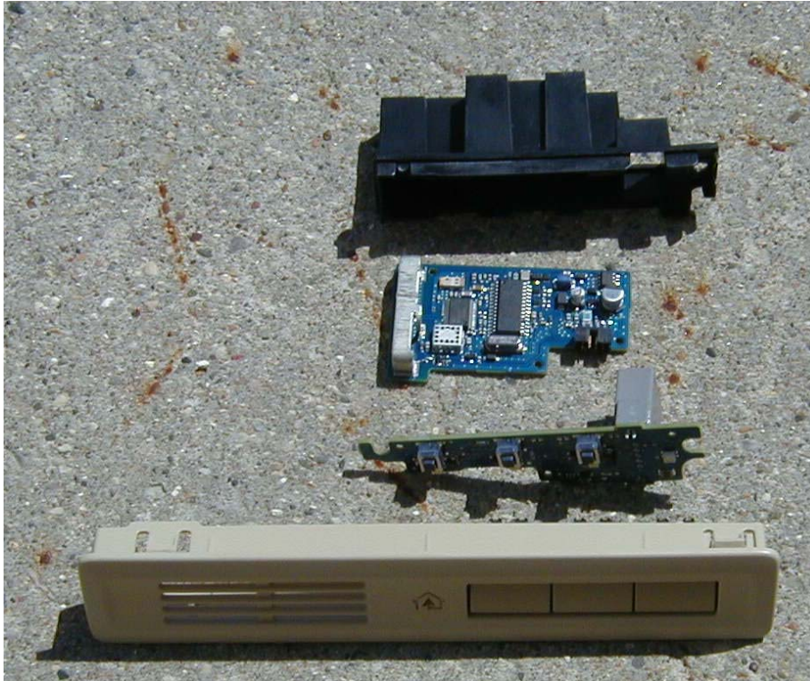
Disassembled View
