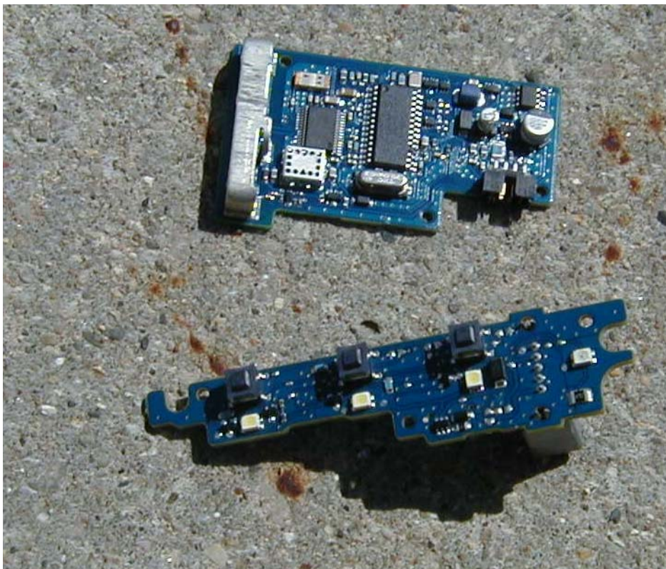
Transceiver and Button PCB, Top View
