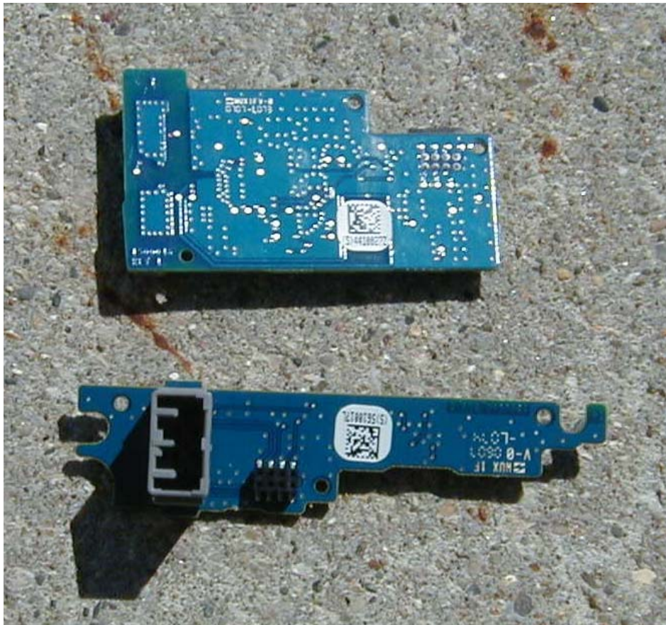
Transceiver and Button PCB, Bottom View
