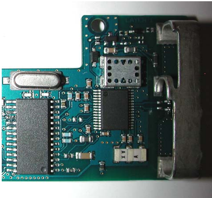
Figure 8.7.3 Close-up of Homelink RF Section.
