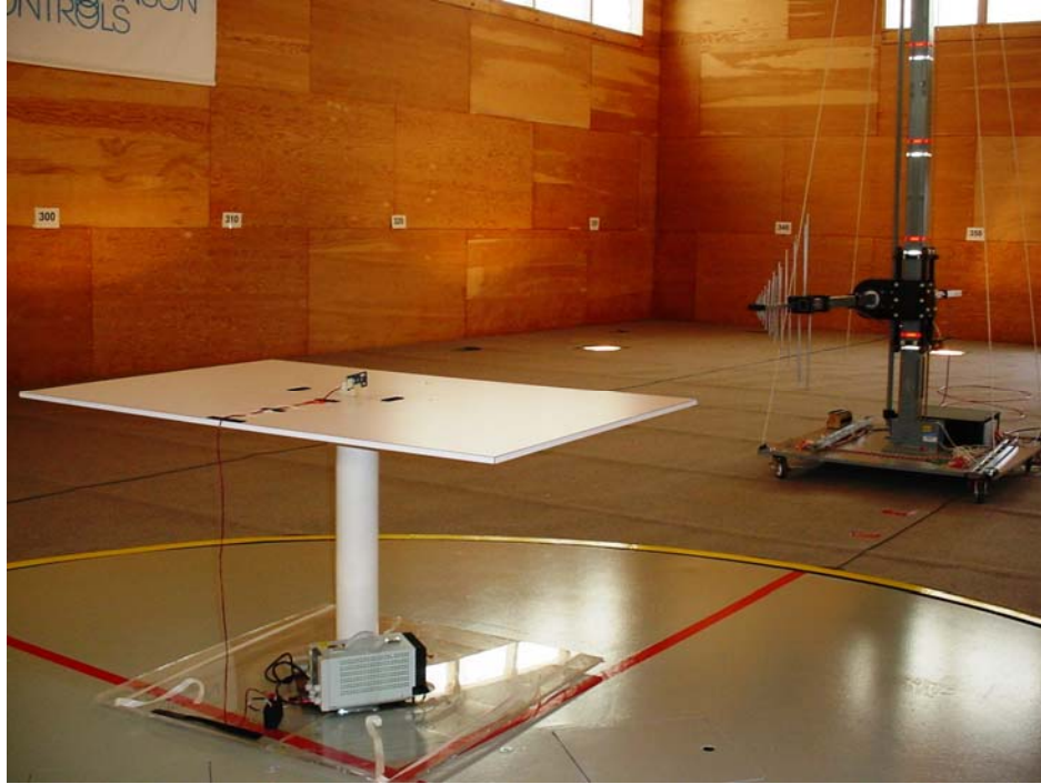
Test Setup - Turntable
