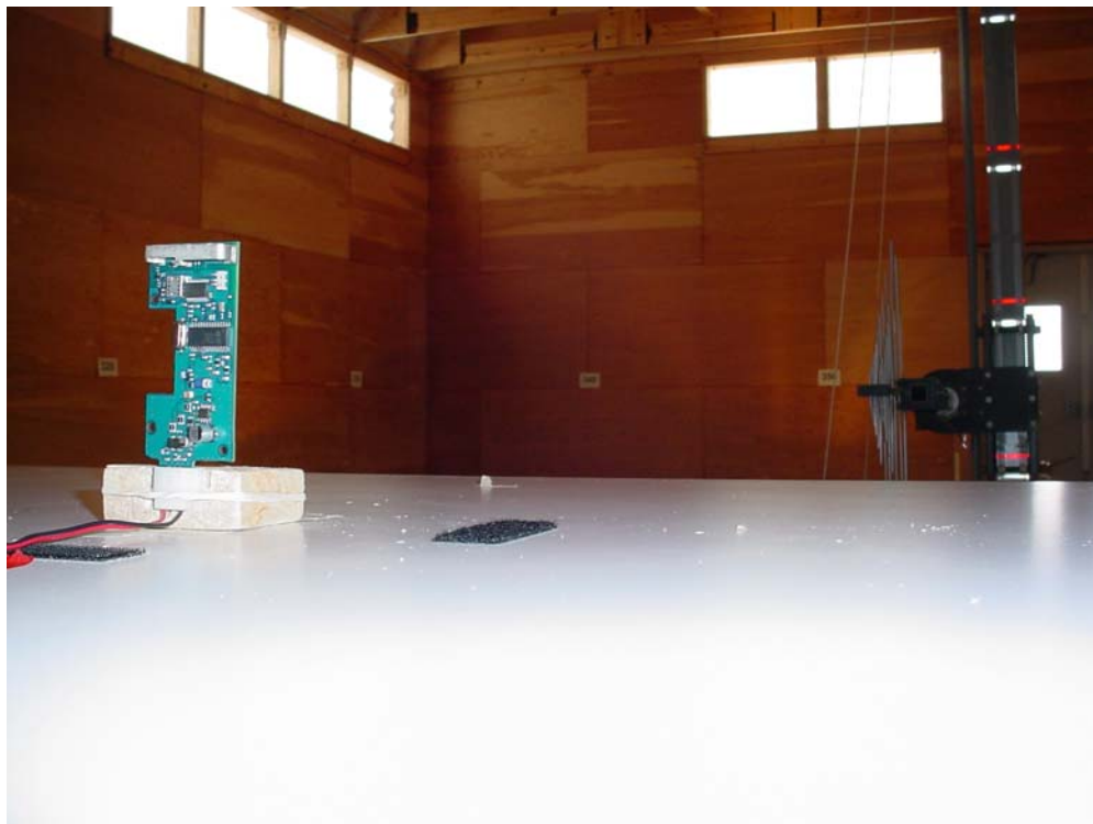
Test Setup – Side View
