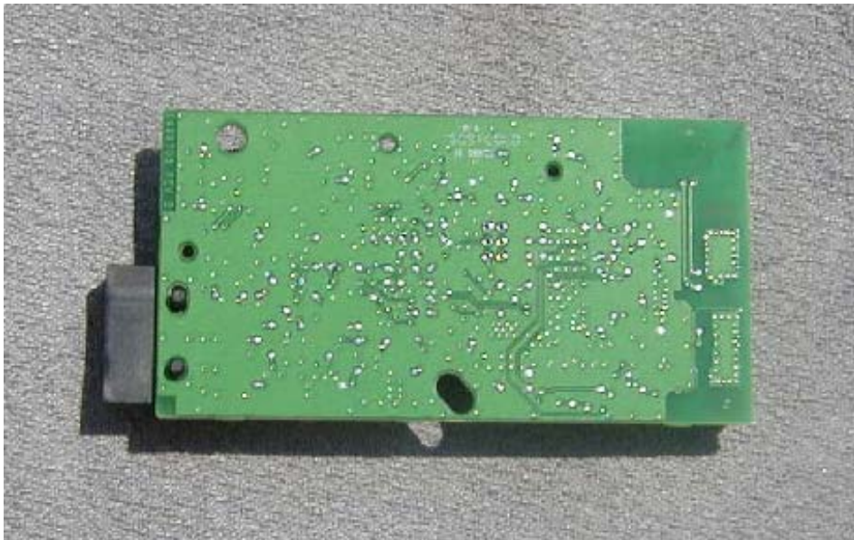
Figure 8.4.2 Internal View, Rear
