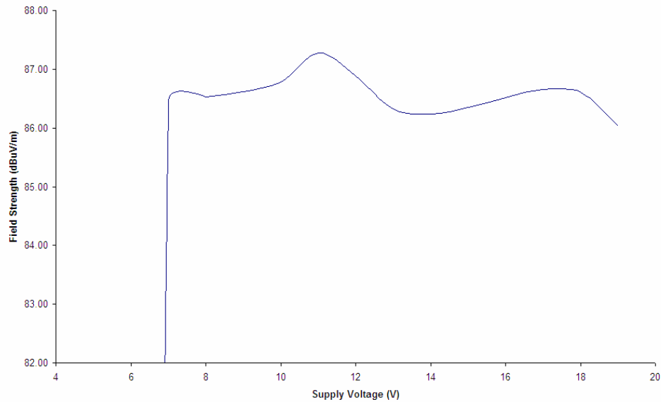
Output Field Strength vs. Supply Voltage
