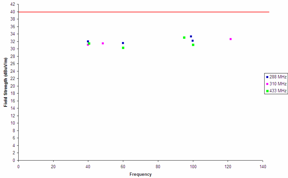
Digital Emissions (Ambients Excluded) by transmitting frequency
