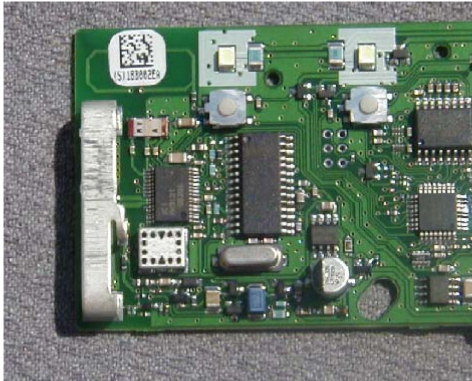
Figure 8.4.1 Close-up of Homelink RF Section.
