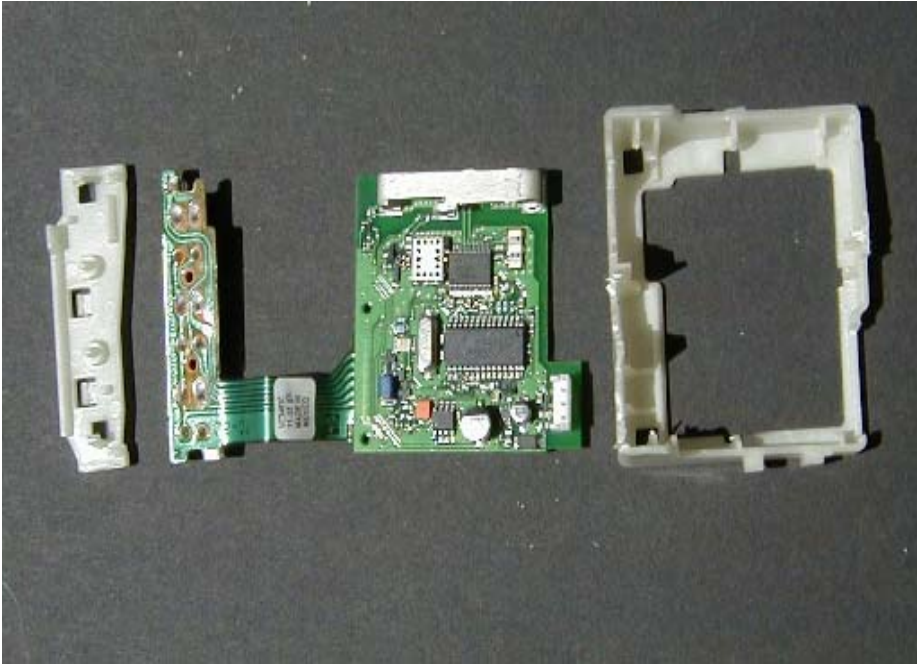
Unit Disassembled
