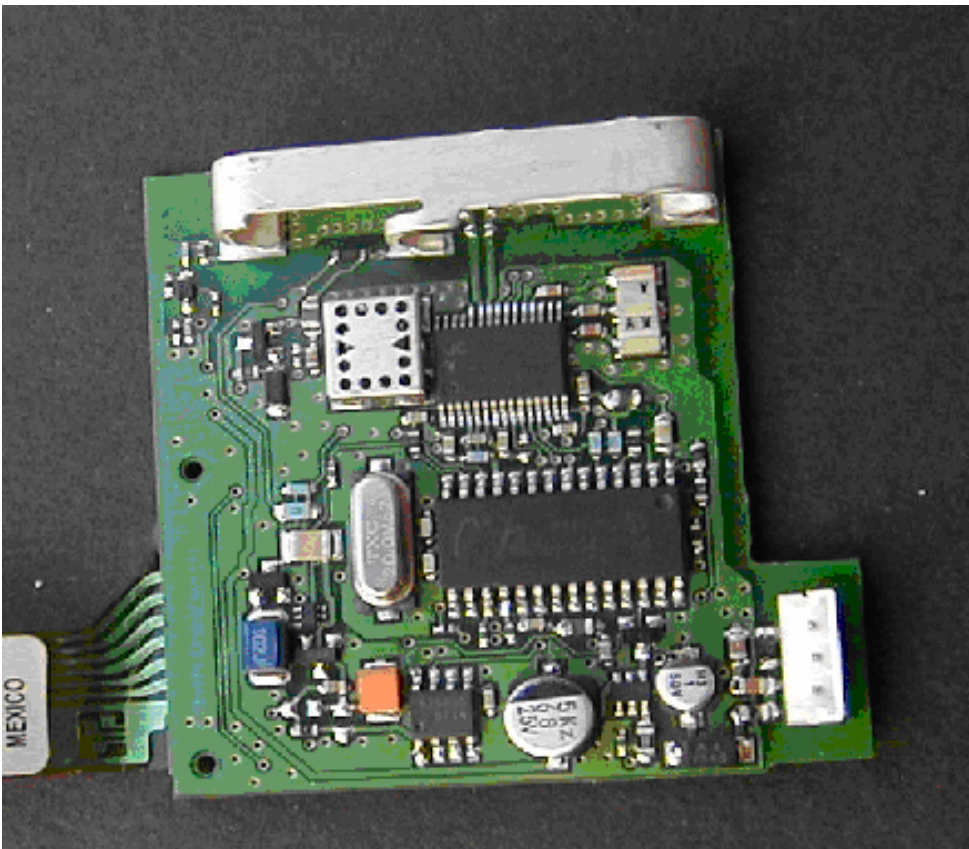
Close-up of Homelink RF Section.
