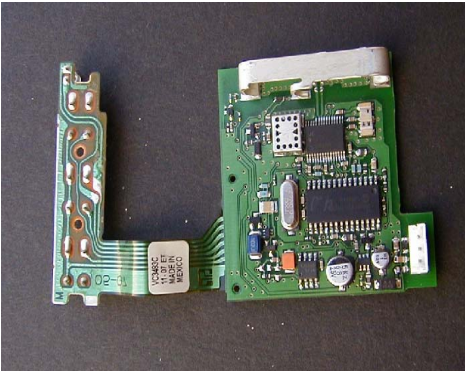
Internal View- Front
