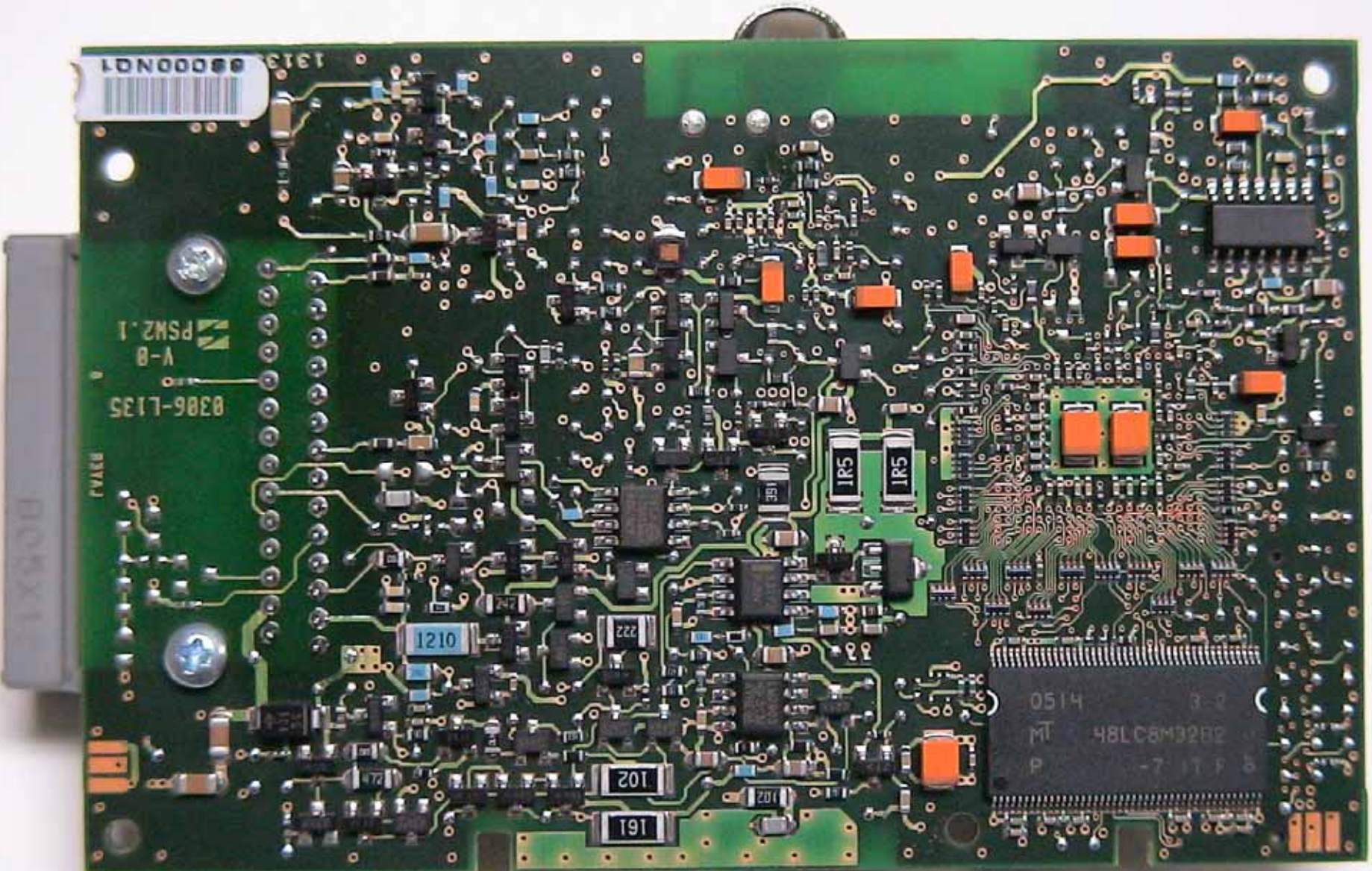
PCB (bottom)
