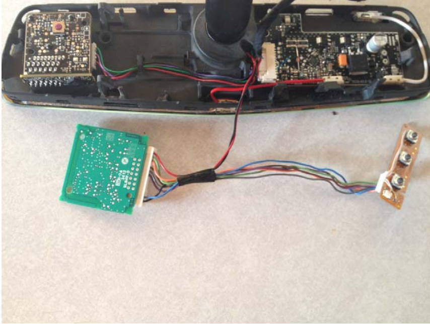
8.3 Close-up of Homelink RF Section.
